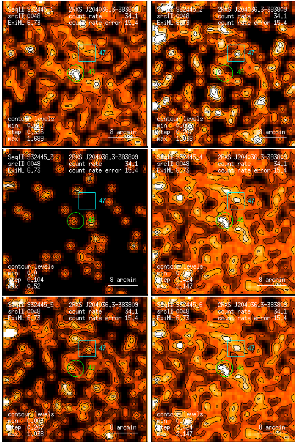
Figure 48: RASS 932445: detection 0048: band rate images, Gaussian filter: (1) PSPC channels 11 – 41, (2) 52 – 90, (3) 91 – 201, (4) 11 – 235, (5) 52 – 201, (6) 11 – 201. Broad band rates in counts/ks. Band rate contour levels in counts/ks/arcmin 2 .
