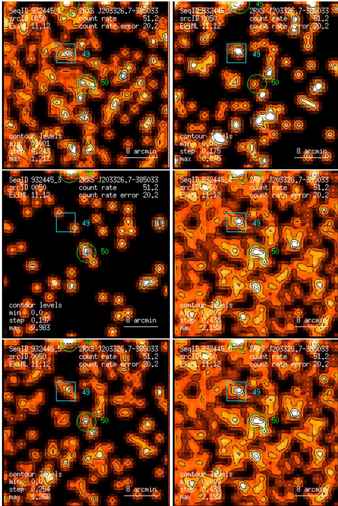
Figure 50: RASS 932445: detection 0050: band rate images, Gaussian filter: (1) PSPC channels 11 – 41, (2) 52 – 90, (3) 91 – 201, (4) 11 – 235, (5) 52 – 201, (6) 11 – 201. Broad band rates in counts/ks. Band rate contour levels in counts/ks/arcmin 2 .
