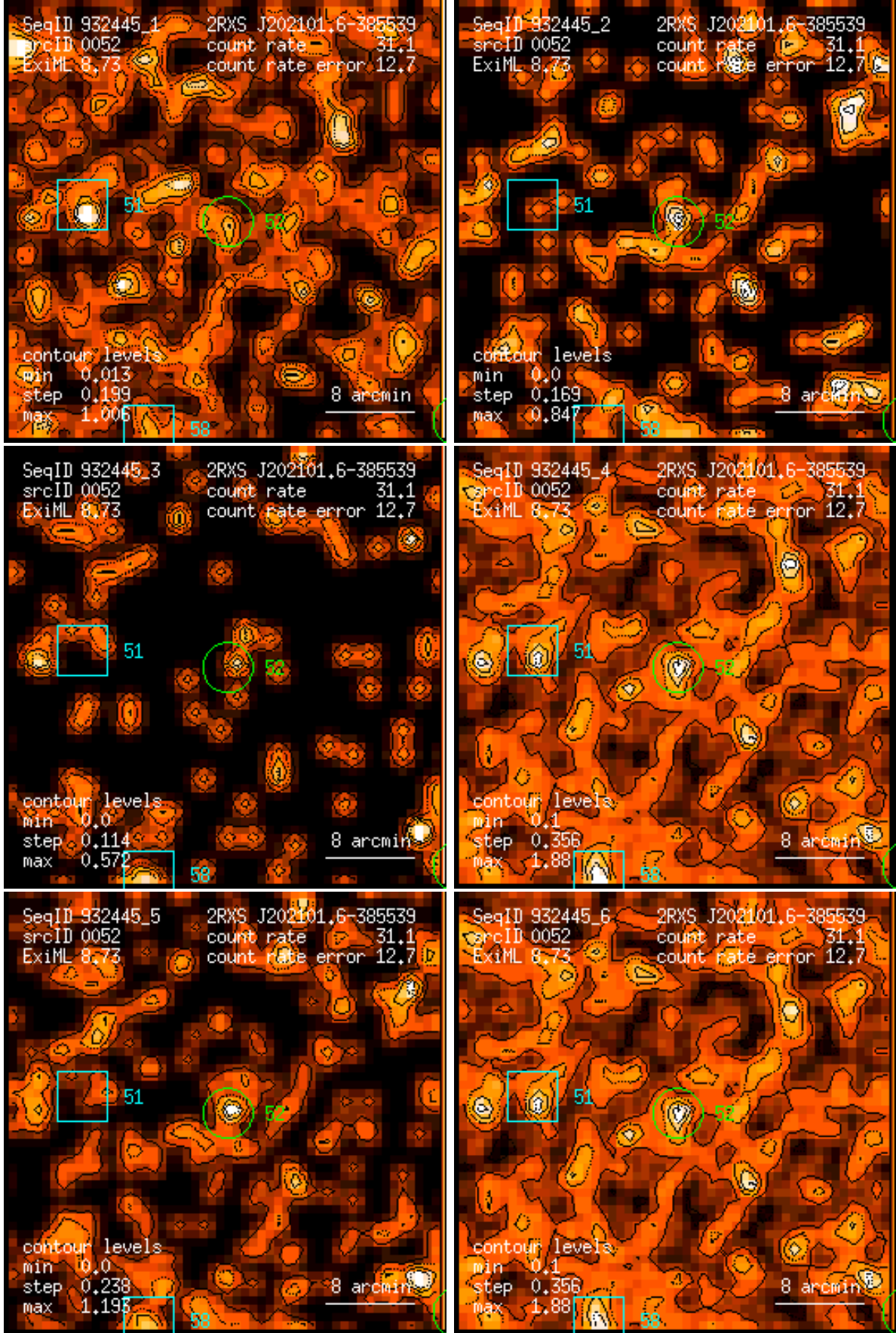
Figure 52: RASS 932445: detection 0052: band rate images, Gaussian filter: (1) PSPC channels 11 – 41, (2) 52 – 90, (3) 91 – 201, (4) 11 – 235, (5) 52 – 201, (6) 11 – 201. Broad band rates in counts/ks. Band rate contour levels in counts/ks/arcmin 2 .
