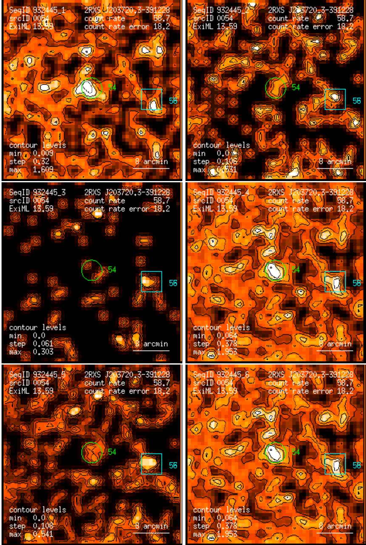
Figure 54: RASS 932445: detection 0054: band rate images, Gaussian filter: (1) PSPC channels 11 – 41, (2) 52 – 90, (3) 91 – 201, (4) 11 – 235, (5) 52 – 201, (6) 11 – 201. Broad band rates in counts/ks. Band rate contour levels in counts/ks/arcmin 2 .
