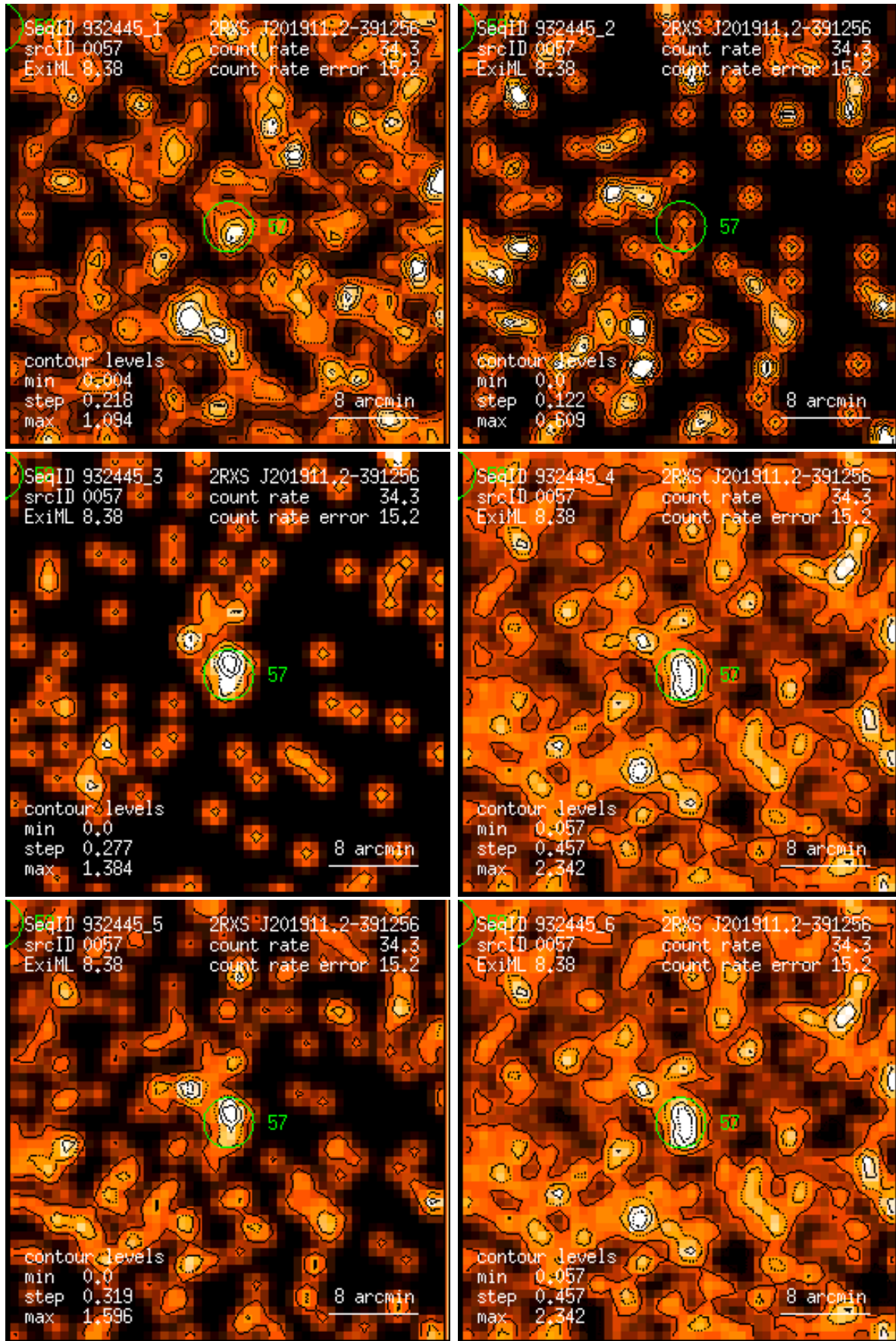
Figure 57: RASS 932445: detection 0057: band rate images, Gaussian filter: (1) PSPC channels 11 – 41, (2) 52 – 90, (3) 91 – 201, (4) 11 – 235, (5) 52 – 201, (6) 11 – 201. Broad band rates in counts/ks. Band rate contour levels in counts/ks/arcmin 2 .
