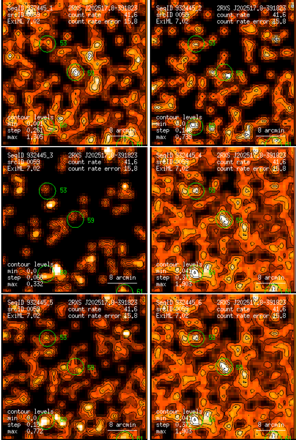
Figure 59: RASS 932445: detection 0059: band rate images, Gaussian filter: (1) PSPC channels 11 – 41, (2) 52 – 90, (3) 91 – 201, (4) 11 – 235, (5) 52 – 201, (6) 11 – 201. Broad band rates in counts/ks. Band rate contour levels in counts/ks/arcmin 2 .
