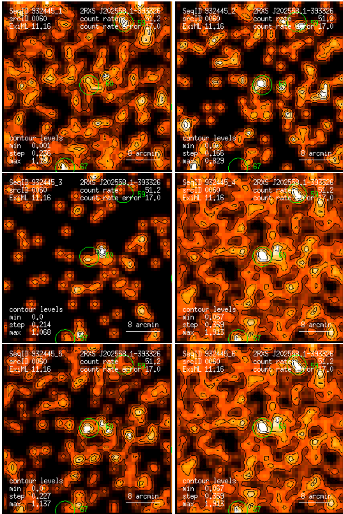
Figure 60: RASS 932445: detection 0060: band rate images, Gaussian filter: (1) PSPC channels 11 – 41, (2) 52 – 90, (3) 91 – 201, (4) 11 – 235, (5) 52 – 201, (6) 11 – 201. Broad band rates in counts/ks. Band rate contour levels in counts/ks/arcmin 2 .
