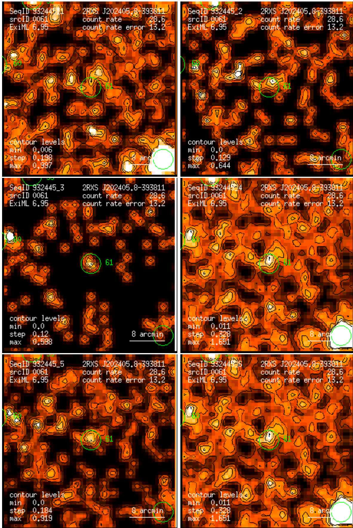
Figure 61: RASS 932445: detection 0061: band rate images, Gaussian filter: (1) PSPC channels 11 – 41, (2) 52 – 90, (3) 91 – 201, (4) 11 – 235, (5) 52 – 201, (6) 11 – 201. Broad band rates in counts/ks. Band rate contour levels in counts/ks/arcmin 2 .
