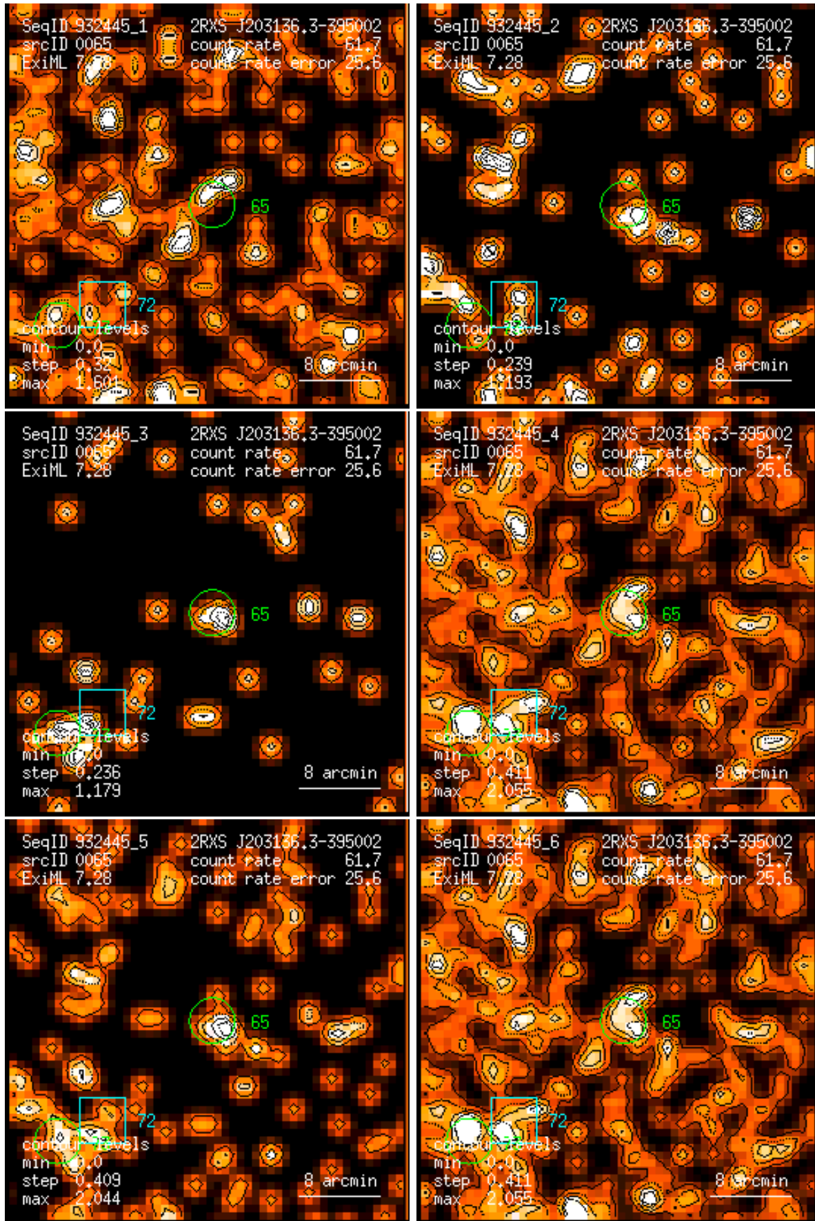
Figure 65: RASS 932445: detection 0065: band rate images, Gaussian filter: (1) PSPC channels 11 – 41, (2) 52 – 90, (3) 91 – 201, (4) 11 – 235, (5) 52 – 201, (6) 11 – 201. Broad band rates in counts/ks. Band rate contour levels in counts/ks/arcmin 2 .
