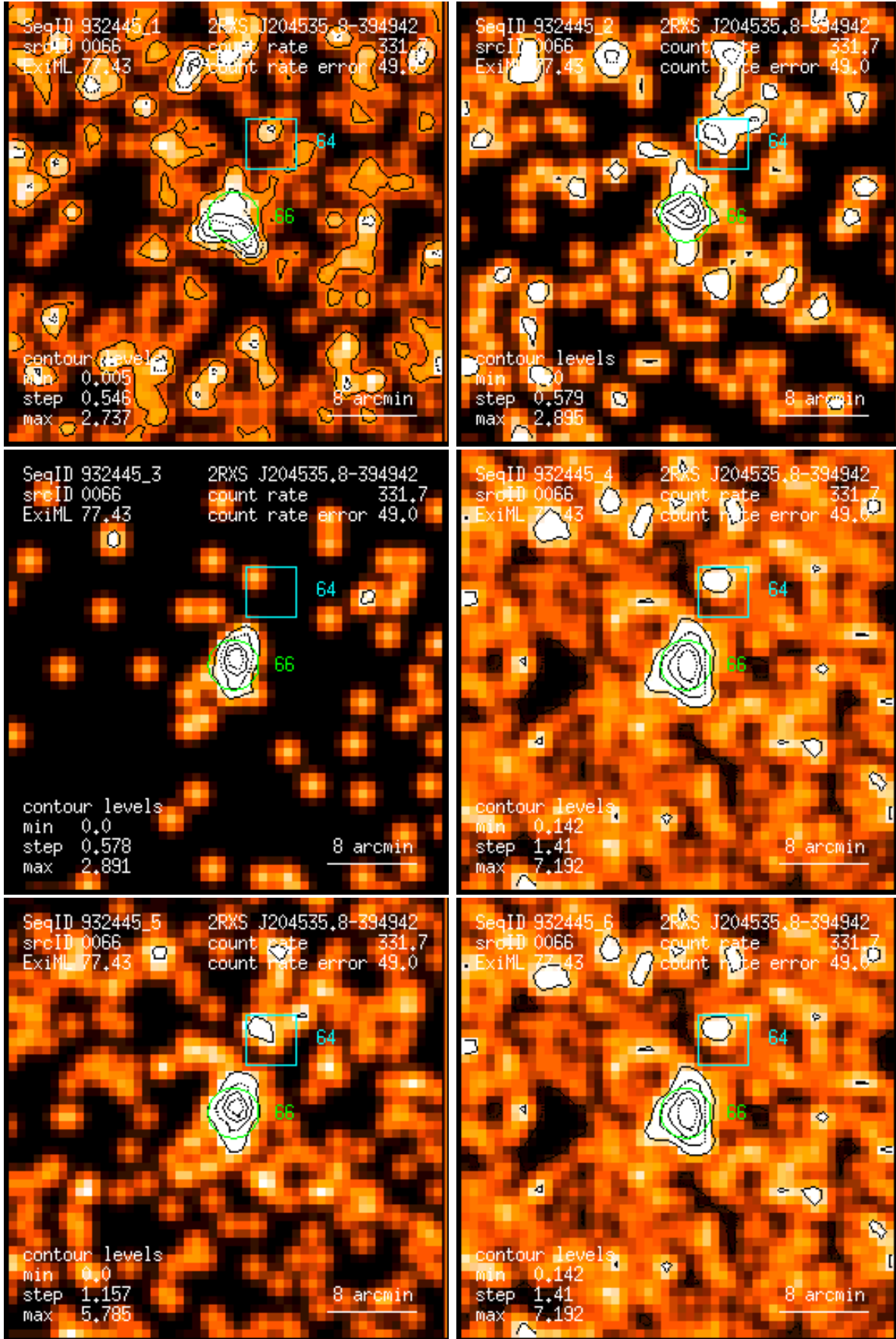
Figure 66: RASS 932445: detection 0066: band rate images, Gaussian filter: (1) PSPC channels 11 – 41, (2) 52 – 90, (3) 91 – 201, (4) 11 – 235, (5) 52 – 201, (6) 11 – 201. Broad band rates in counts/ks. Band rate contour levels in counts/ks/arcmin 2 .
