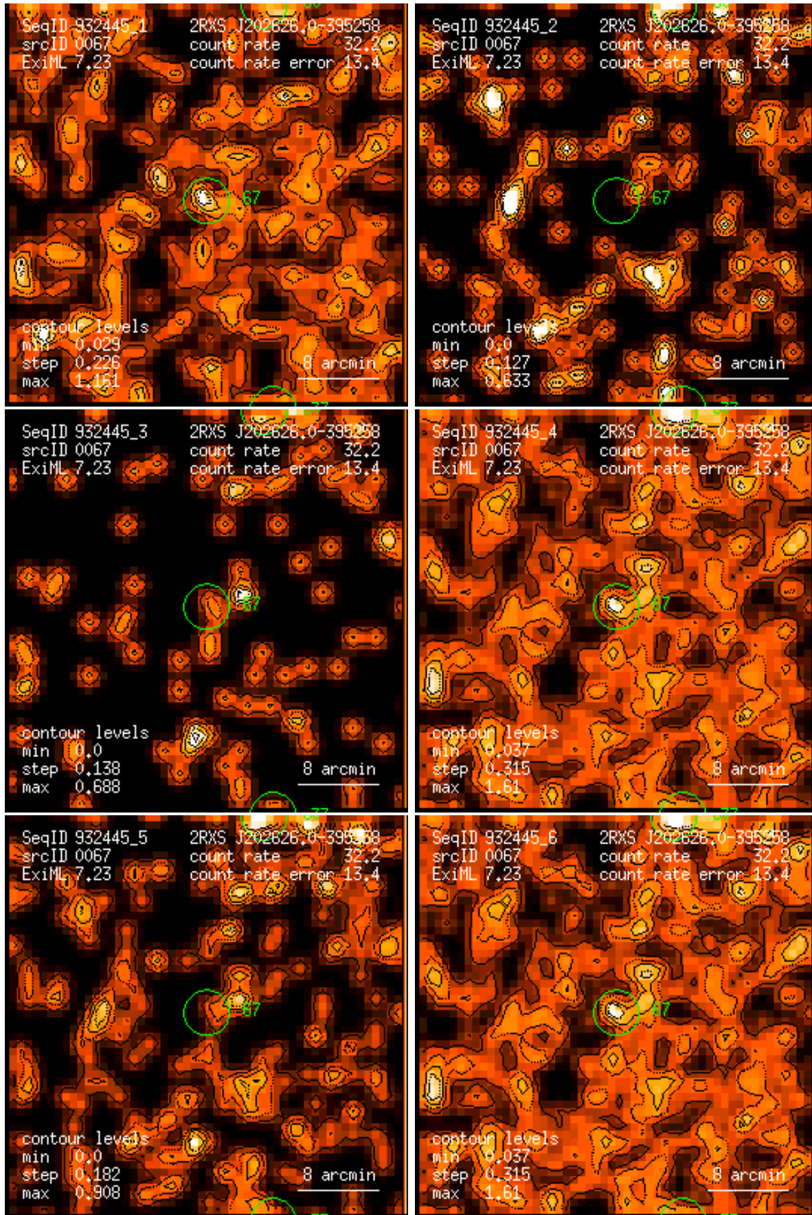
Figure 67: RASS 932445: detection 0067: band rate images, Gaussian filter: (1) PSPC channels 11 – 41, (2) 52 – 90, (3) 91 – 201, (4) 11 – 235, (5) 52 – 201, (6) 11 – 201. Broad band rates in counts/ks. Band rate contour levels in counts/ks/arcmin 2 .
