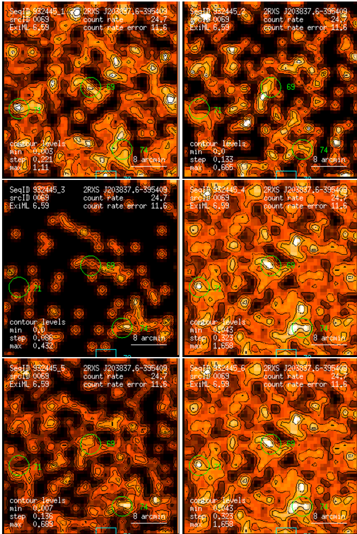
Figure 69: RASS 932445: detection 0069: band rate images, Gaussian filter: (1) PSPC channels 11 – 41, (2) 52 – 90, (3) 91 – 201, (4) 11 – 235, (5) 52 – 201, (6) 11 – 201. Broad band rates in counts/ks. Band rate contour levels in counts/ks/arcmin 2 .
