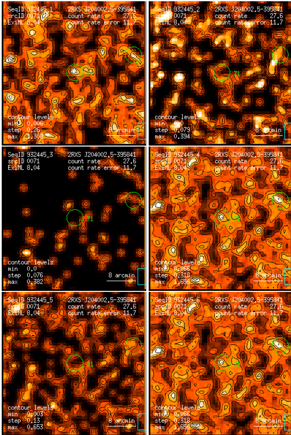
Figure 71: RASS 932445: detection 0071: band rate images, Gaussian filter: (1) PSPC channels 11 – 41, (2) 52 – 90, (3) 91 – 201, (4) 11 – 235, (5) 52 – 201, (6) 11 – 201. Broad band rates in counts/ks. Band rate contour levels in counts/ks/arcmin 2 .
