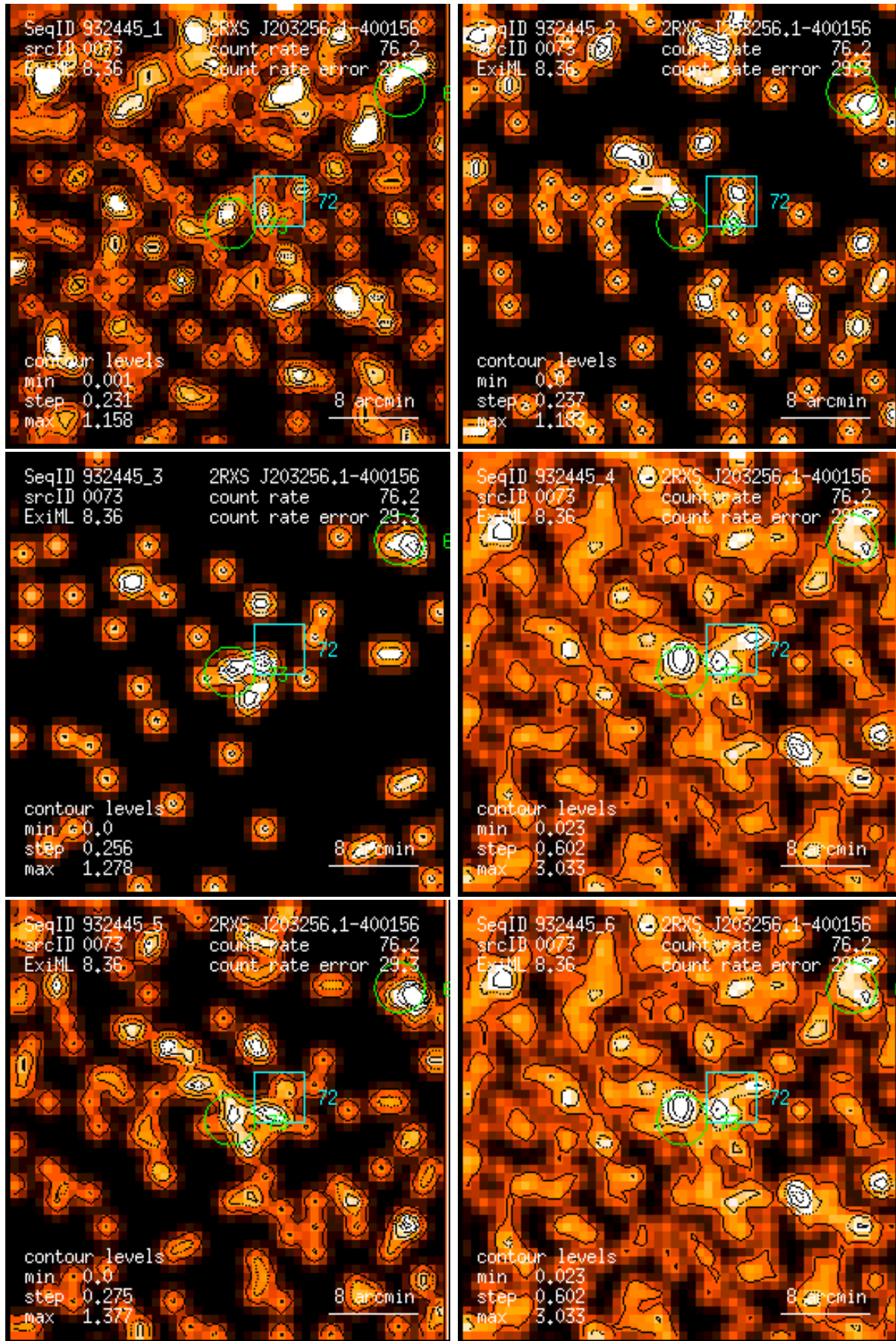
Figure 73: RASS 932445: detection 0073: band rate images, Gaussian filter: (1) PSPC channels 11 – 41, (2) 52 – 90, (3) 91 – 201, (4) 11 – 235, (5) 52 – 201, (6) 11 – 201. Broad band rates in counts/ks. Band rate contour levels in counts/ks/arcmin 2 .
