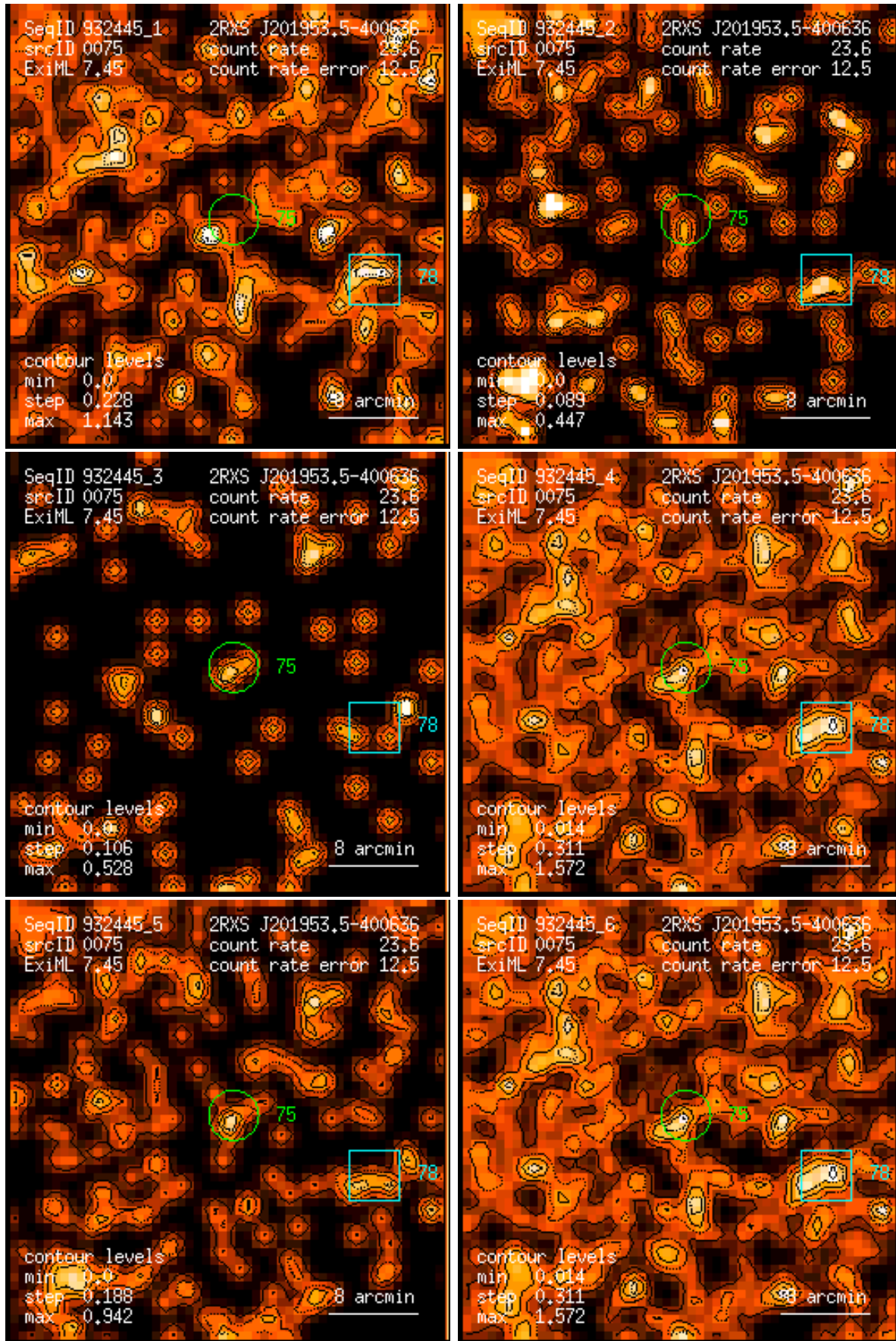
Figure 75: RASS 932445: detection 0075: band rate images, Gaussian filter: (1) PSPC channels 11 – 41, (2) 52 – 90, (3) 91 – 201, (4) 11 – 235, (5) 52 – 201, (6) 11 – 201. Broad band rates in counts/ks. Band rate contour levels in counts/ks/arcmin 2 .
