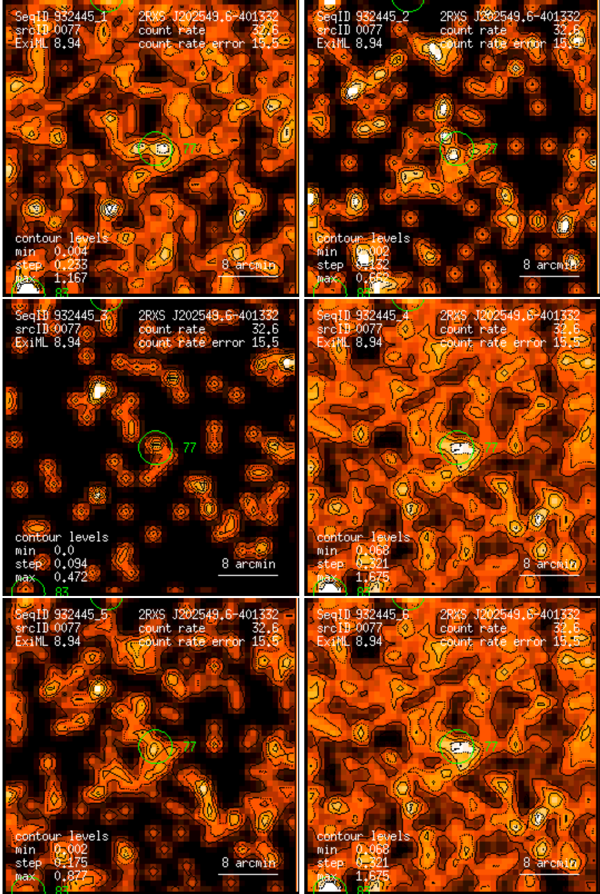
Figure 77: RASS 932445: detection 0077: band rate images, Gaussian filter: (1) PSPC channels 11 – 41, (2) 52 – 90, (3) 91 – 201, (4) 11 – 235, (5) 52 – 201, (6) 11 – 201. Broad band rates in counts/ks. Band rate contour levels in counts/ks/arcmin 2 .
