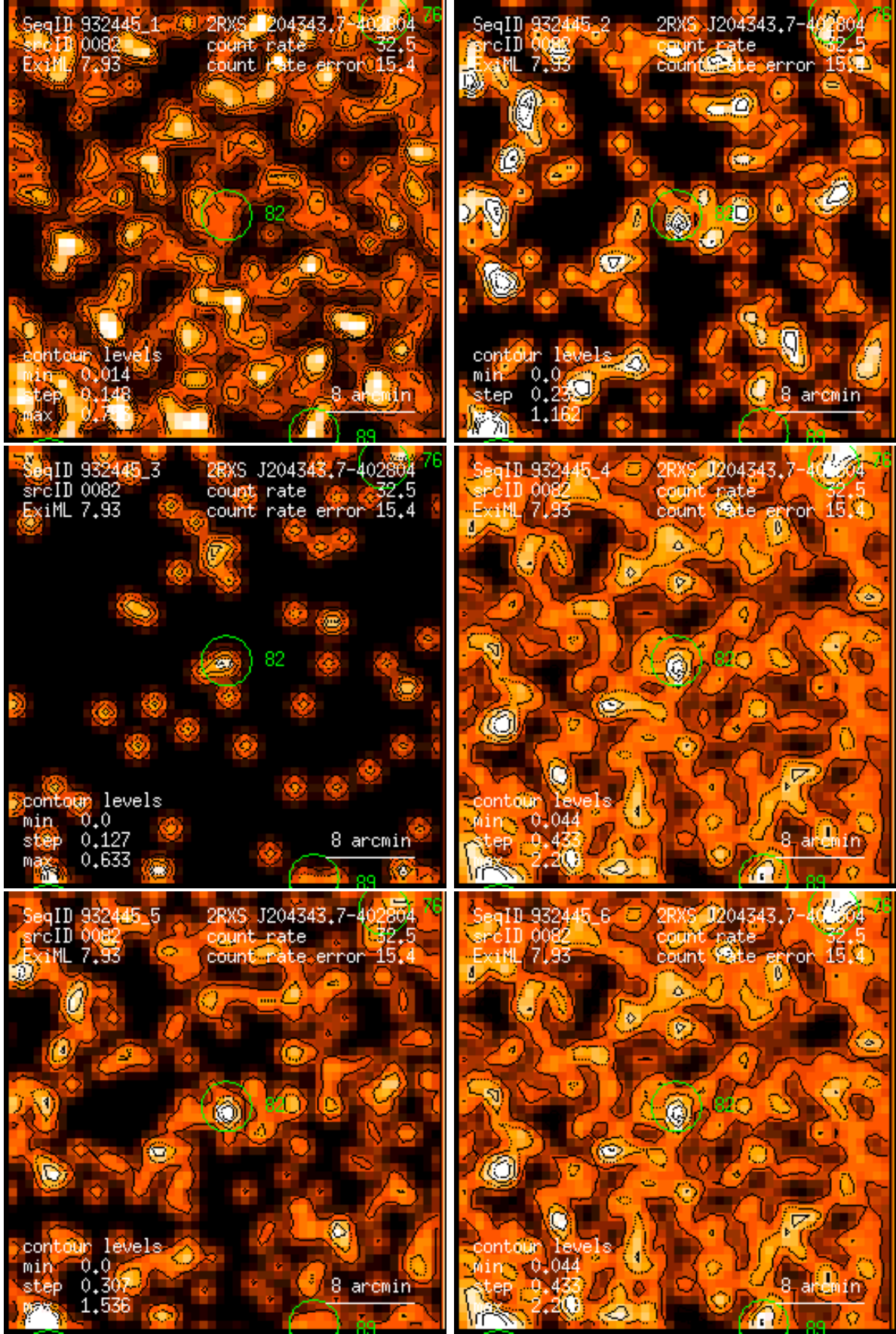
Figure 82: RASS 932445: detection 0082: band rate images, Gaussian filter: (1) PSPC channels 11 – 41, (2) 52 – 90, (3) 91 – 201, (4) 11 – 235, (5) 52 – 201, (6) 11 – 201. Broad band rates in counts/ks. Band rate contour levels in counts/ks/arcmin 2 .
