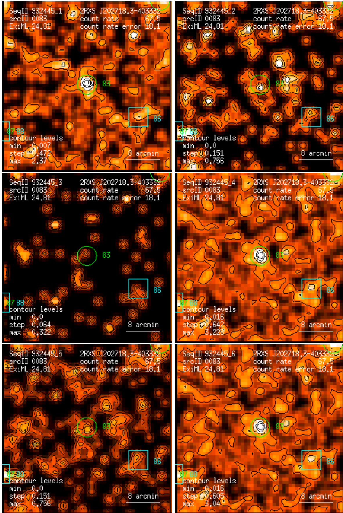
Figure 83: RASS 932445: detection 0083: band rate images, Gaussian filter: (1) PSPC channels 11 – 41, (2) 52 – 90, (3) 91 – 201, (4) 11 – 235, (5) 52 – 201, (6) 11 – 201. Broad band rates in counts/ks. Band rate contour levels in counts/ks/arcmin 2 .
