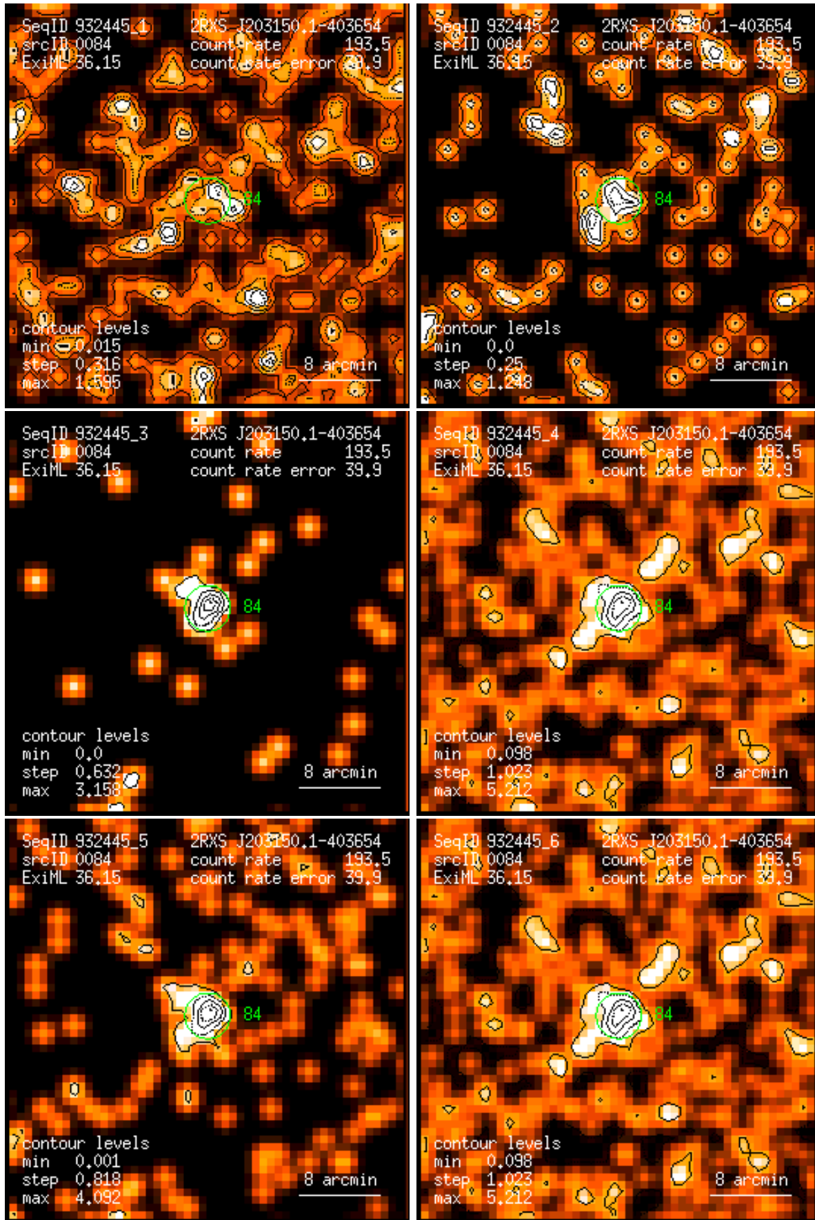
Figure 84: RASS 932445: detection 0084: band rate images, Gaussian filter: (1) PSPC channels 11 – 41, (2) 52 – 90, (3) 91 – 201, (4) 11 – 235, (5) 52 – 201, (6) 11 – 201. Broad band rates in counts/ks. Band rate contour levels in counts/ks/arcmin 2 .
