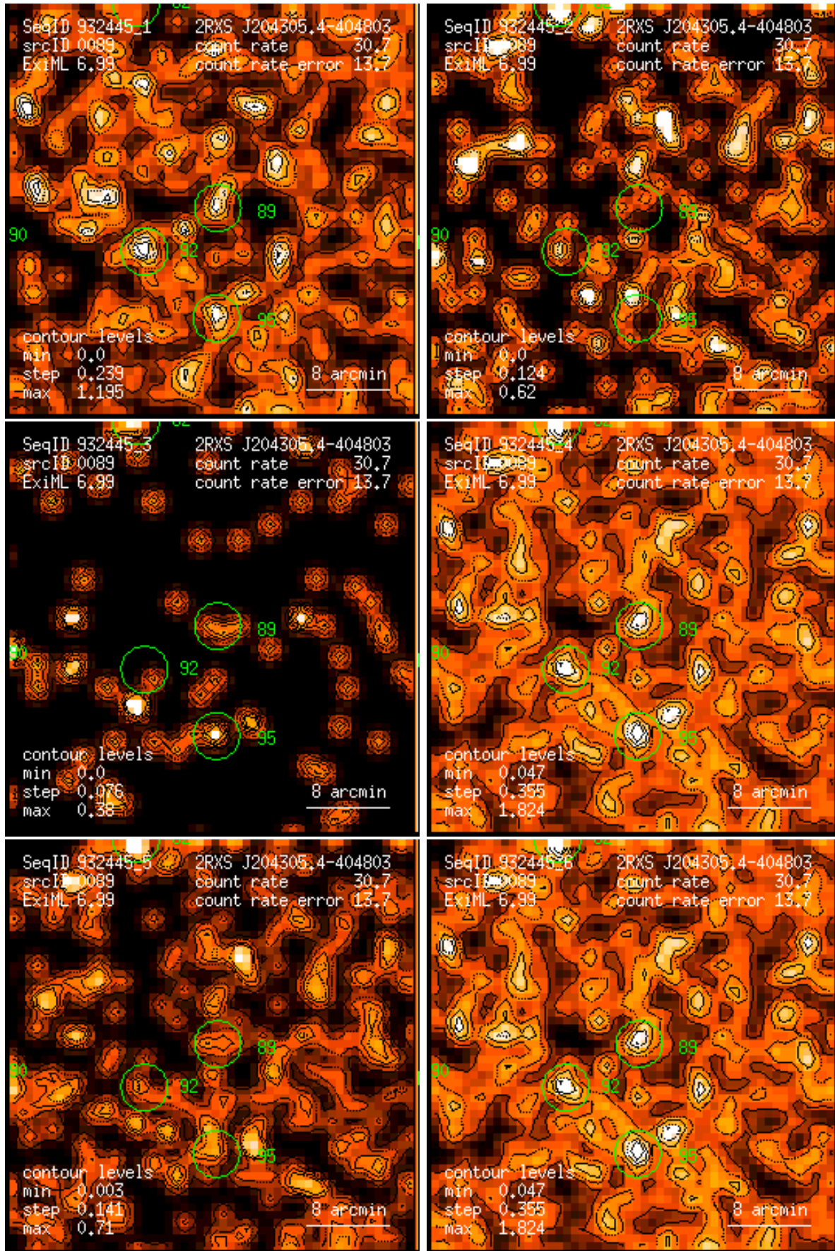
Figure 89: RASS 932445: detection 0089: band rate images, Gaussian filter: (1) PSPC channels 11 – 41, (2) 52 – 90, (3) 91 – 201, (4) 11 – 235, (5) 52 – 201, (6) 11 – 201. Broad band rates in counts/ks. Band rate contour levels in counts/ks/arcmin 2 .
