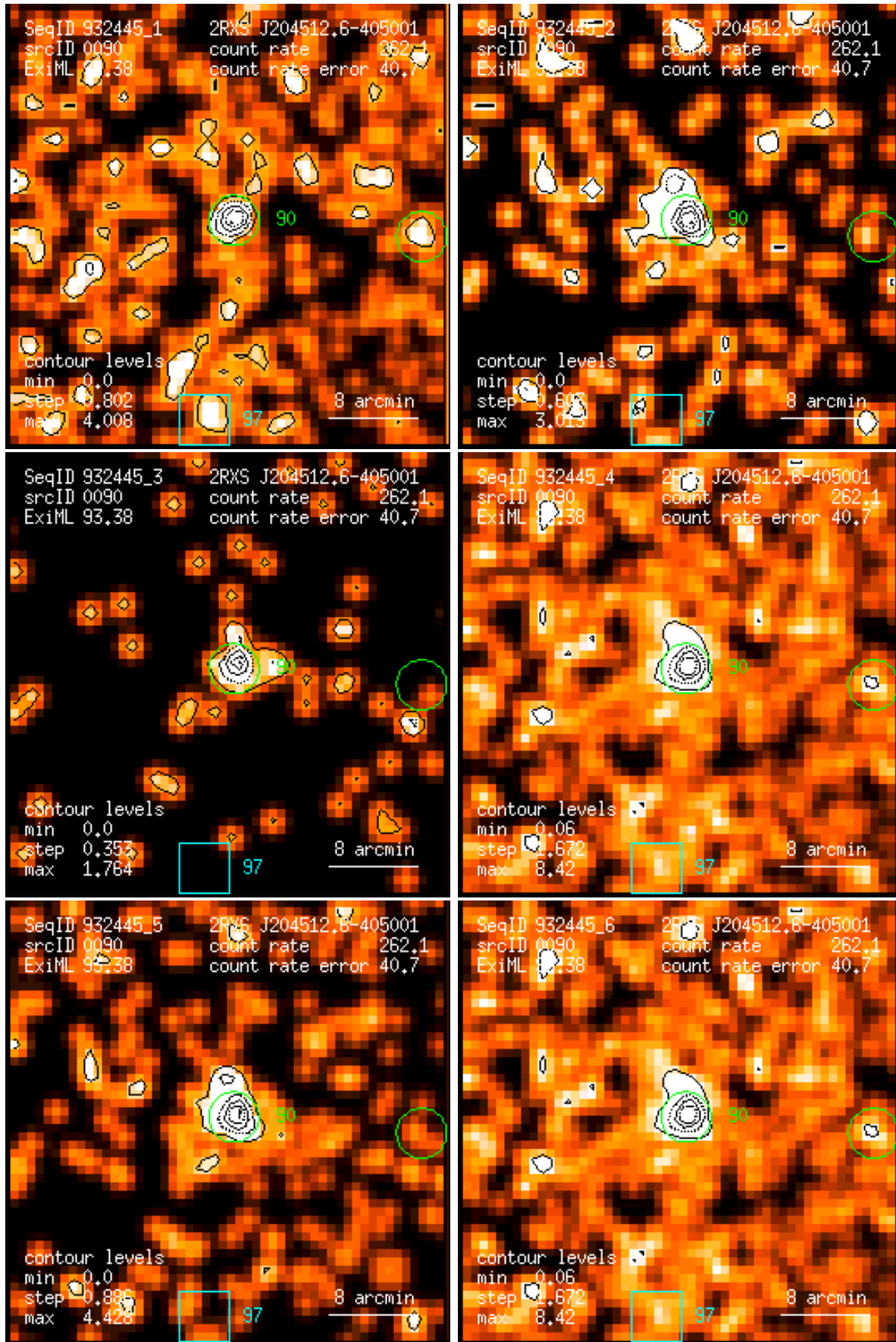
Figure 90: RASS 932445: detection 0090: band rate images, Gaussian filter: (1) PSPC channels 11 – 41, (2) 52 – 90, (3) 91 – 201, (4) 11 – 235, (5) 52 – 201, (6) 11 – 201. Broad band rates in counts/ks. Band rate contour levels in counts/ks/arcmin 2 .
