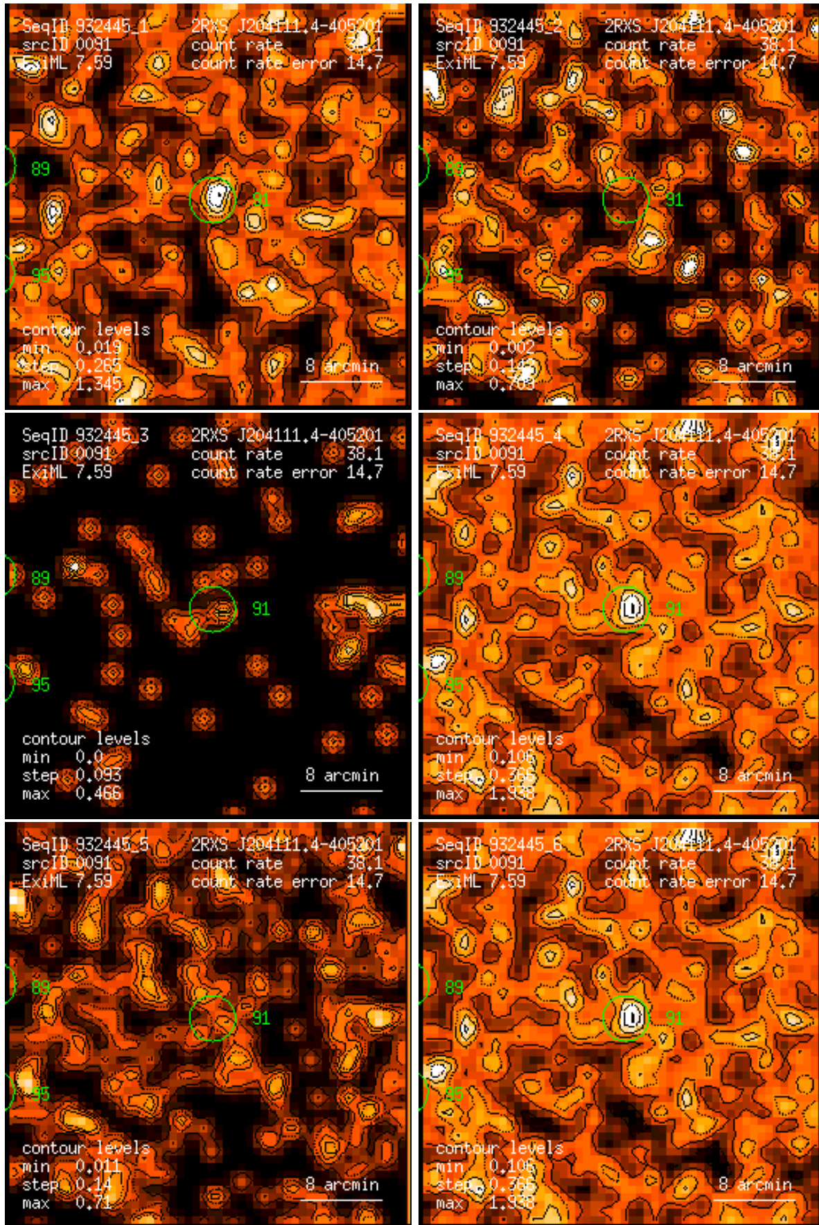
Figure 91: RASS 932445: detection 0091: band rate images, Gaussian filter: (1) PSPC channels 11 – 41, (2) 52 – 90, (3) 91 – 201, (4) 11 – 235, (5) 52 – 201, (6) 11 – 201. Broad band rates in counts/ks. Band rate contour levels in counts/ks/arcmin 2 .
