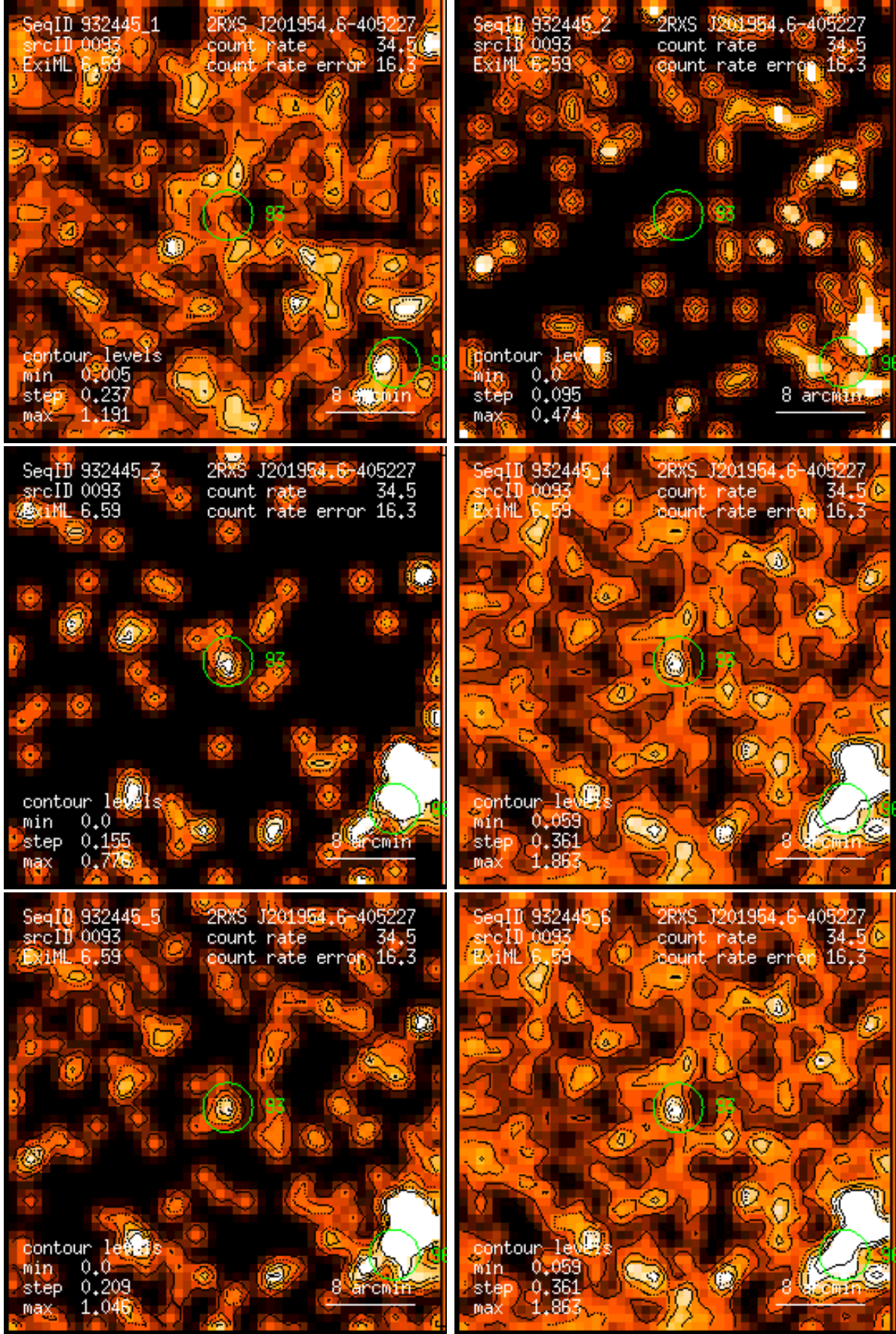
Figure 93: RASS 932445: detection 0093: band rate images, Gaussian filter: (1) PSPC channels 11 – 41, (2) 52 – 90, (3) 91 – 201, (4) 11 – 235, (5) 52 – 201, (6) 11 – 201. Broad band rates in counts/ks. Band rate contour levels in counts/ks/arcmin 2 .
