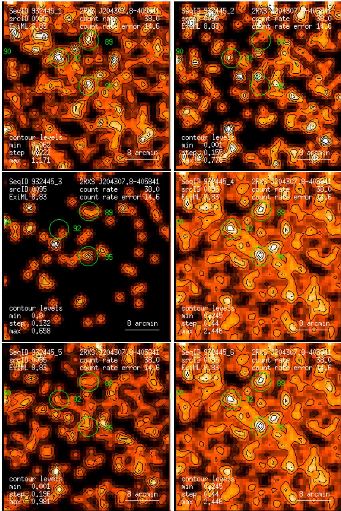
Figure 95: RASS 932445: detection 0095: band rate images, Gaussian filter: (1) PSPC channels 11 – 41, (2) 52 – 90, (3) 91 – 201, (4) 11 – 235, (5) 52 – 201, (6) 11 – 201. Broad band rates in counts/ks. Band rate contour levels in counts/ks/arcmin 2 .
