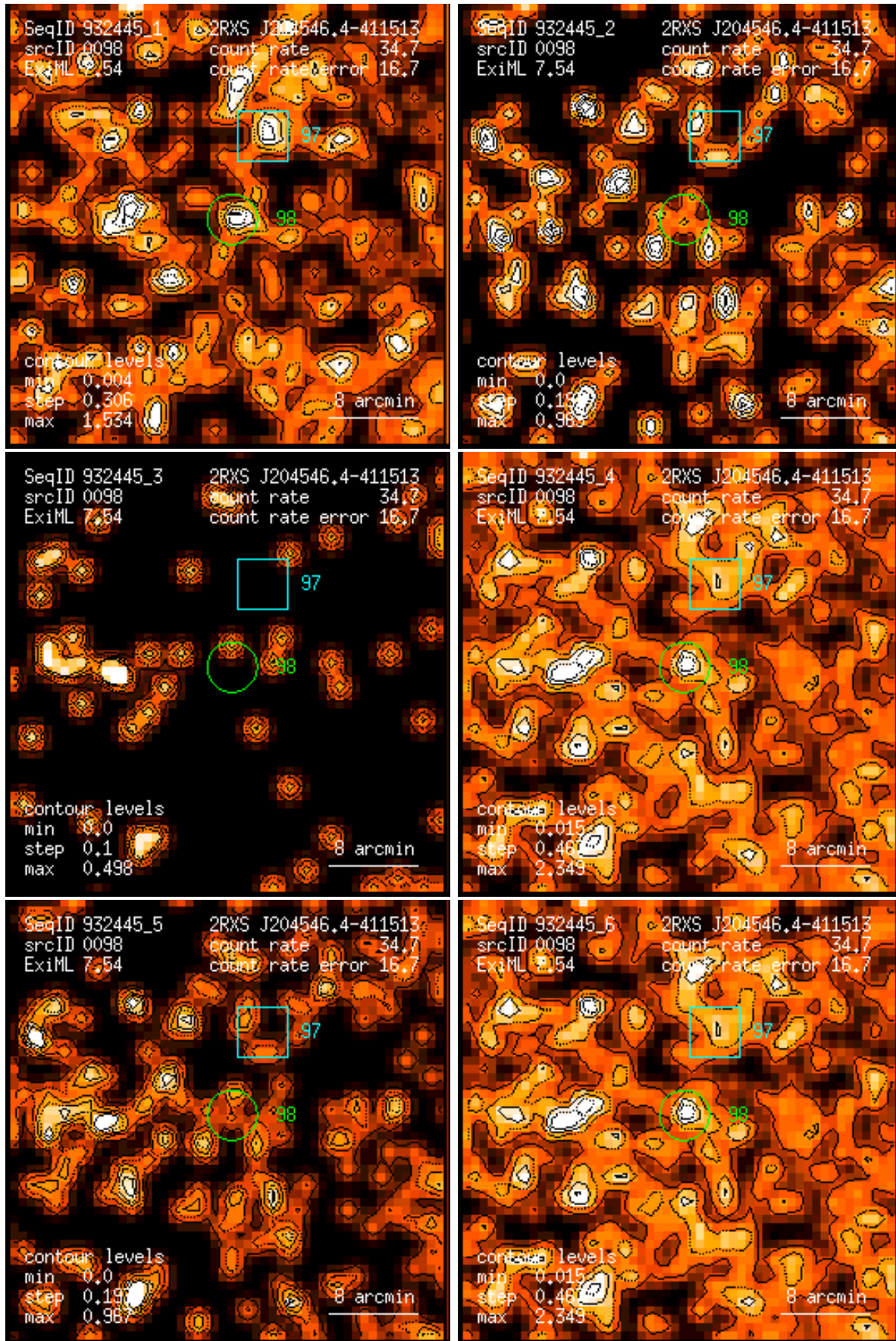
Figure 98: RASS 932445: detection 0098: band rate images, Gaussian filter: (1) PSPC channels 11 – 41, (2) 52 – 90, (3) 91 – 201, (4) 11 – 235, (5) 52 – 201, (6) 11 – 201. Broad band rates in counts/ks. Band rate contour levels in counts/ks/arcmin 2 .
