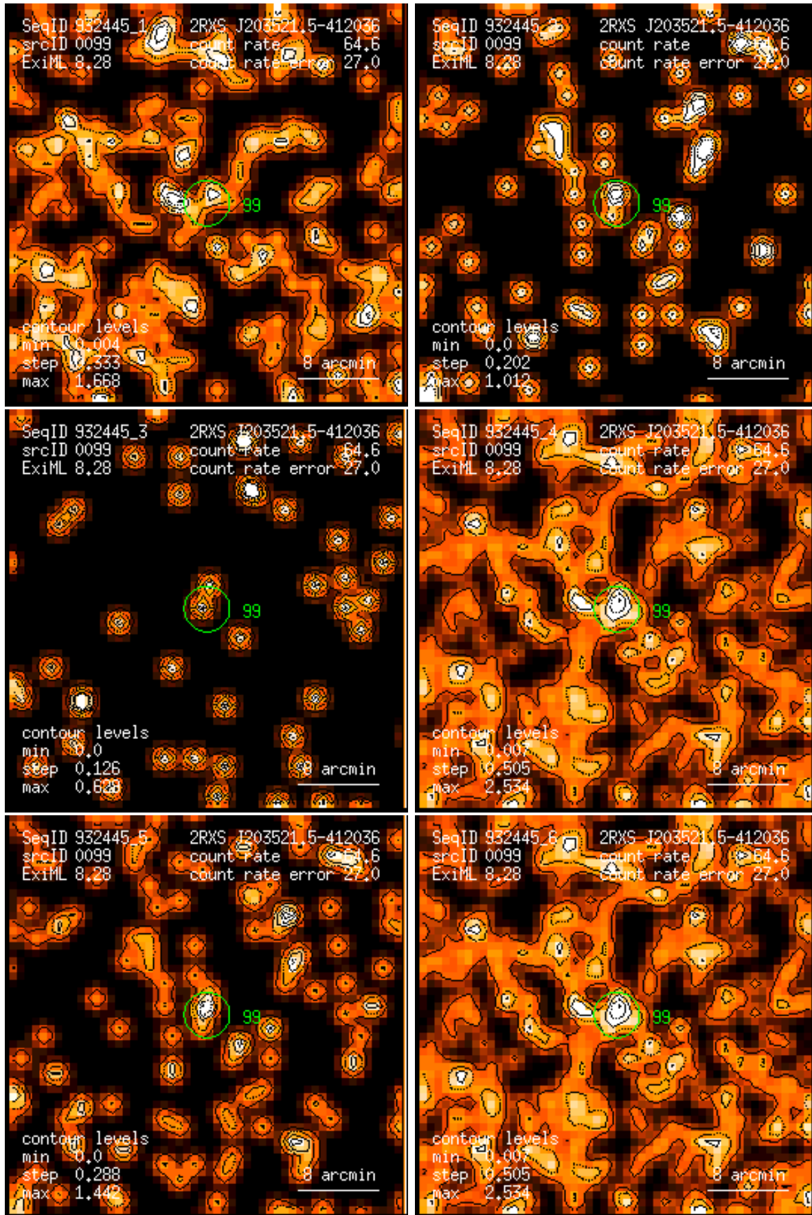
Figure 99: RASS 932445: detection 0099: band rate images, Gaussian filter: (1) PSPC channels 11 – 41, (2) 52 – 90, (3) 91 – 201, (4) 11 – 235, (5) 52 – 201, (6) 11 – 201. Broad band rates in counts/ks. Band rate contour levels in counts/ks/arcmin 2 .
