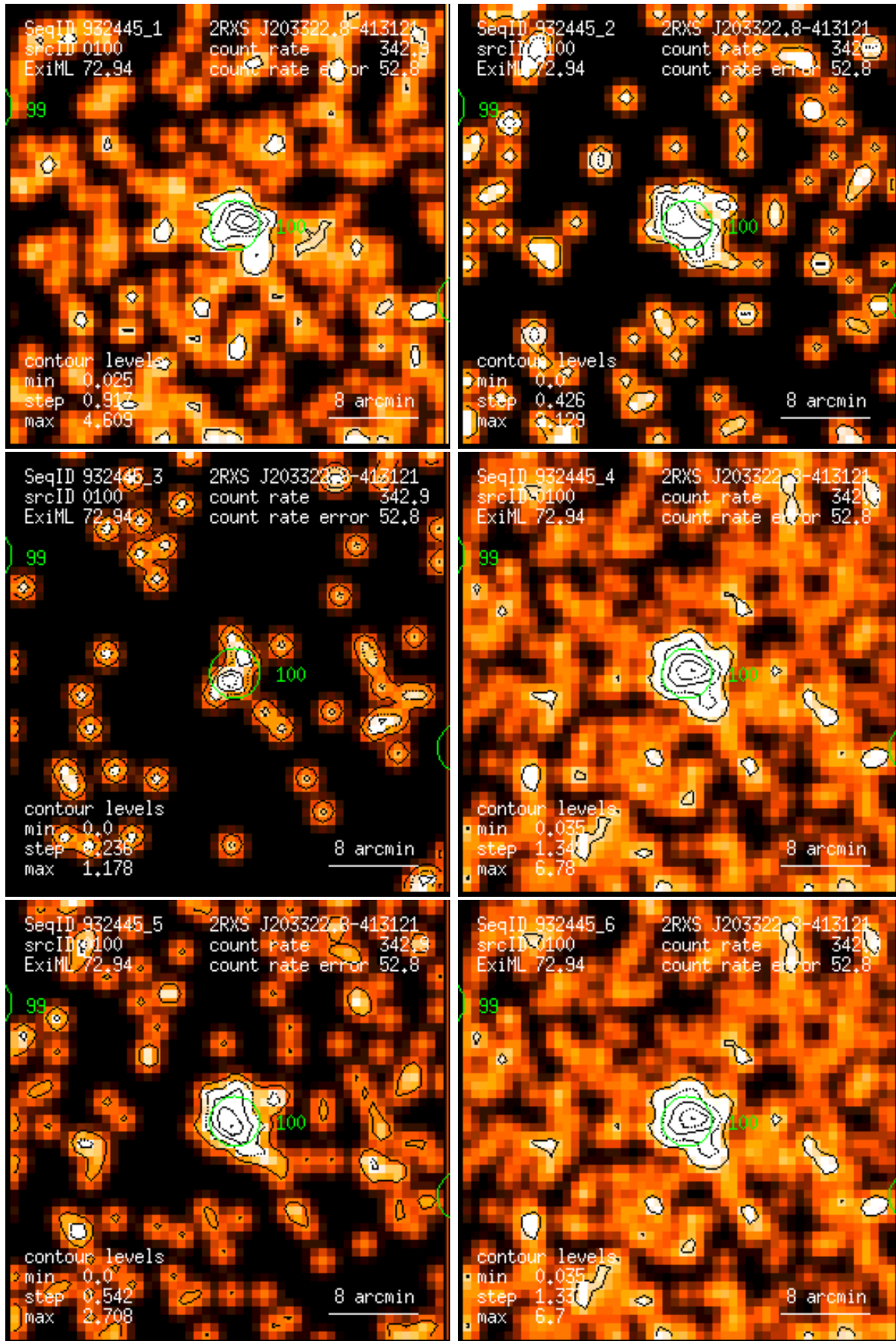
Figure 100: RASS 932445: detection 0100: band rate images, Gaussian filter: (1) PSPC channels 11 – 41, (2) 52 – 90, (3) 91 – 201, (4) 11 – 235, (5) 52 – 201, (6) 11 – 201. Broad band rates in counts/ks. Band rate contour levels in counts/ks/arcmin 2 .
