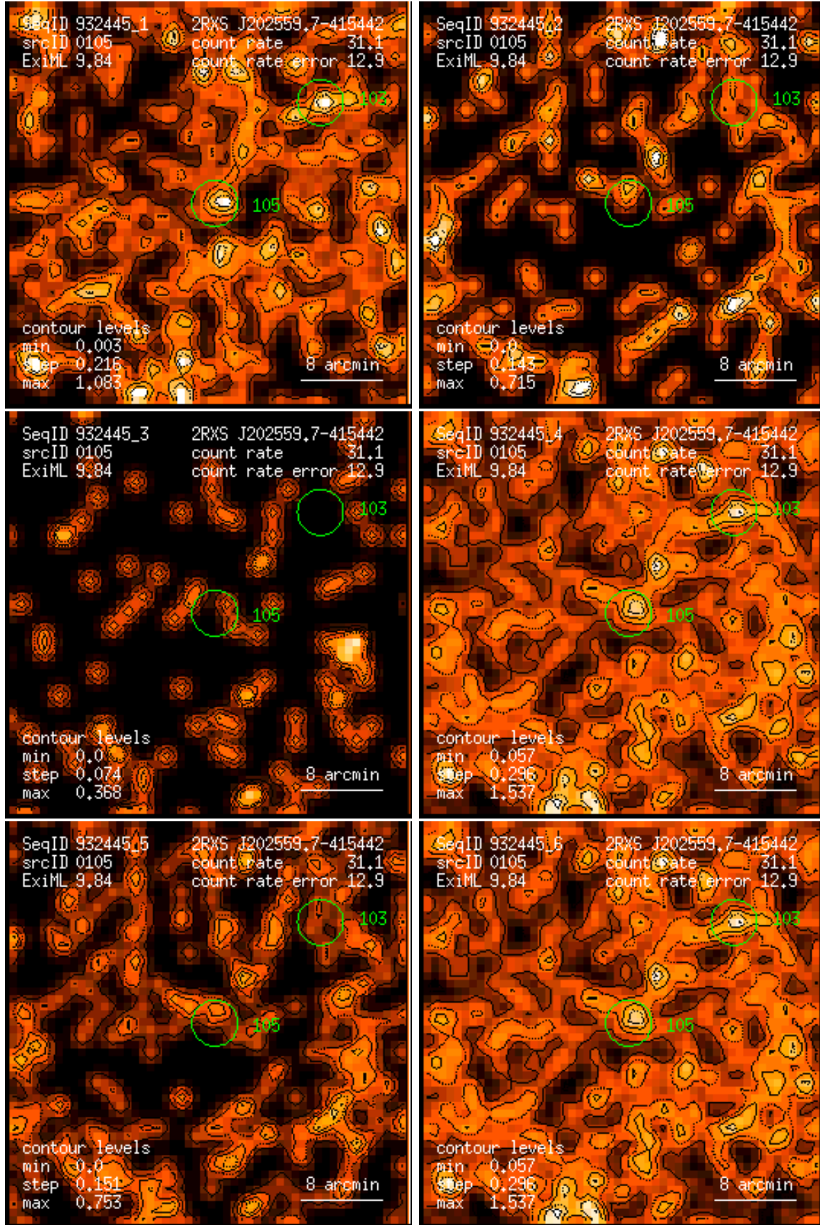
Figure 105: RASS 932445: detection 0105: band rate images, Gaussian filter: (1) PSPC channels 11 – 41, (2) 52 – 90, (3) 91 – 201, (4) 11 – 235, (5) 52 – 201, (6) 11 – 201. Broad band rates in counts/ks. Band rate contour levels in counts/ks/arcmin 2 .
