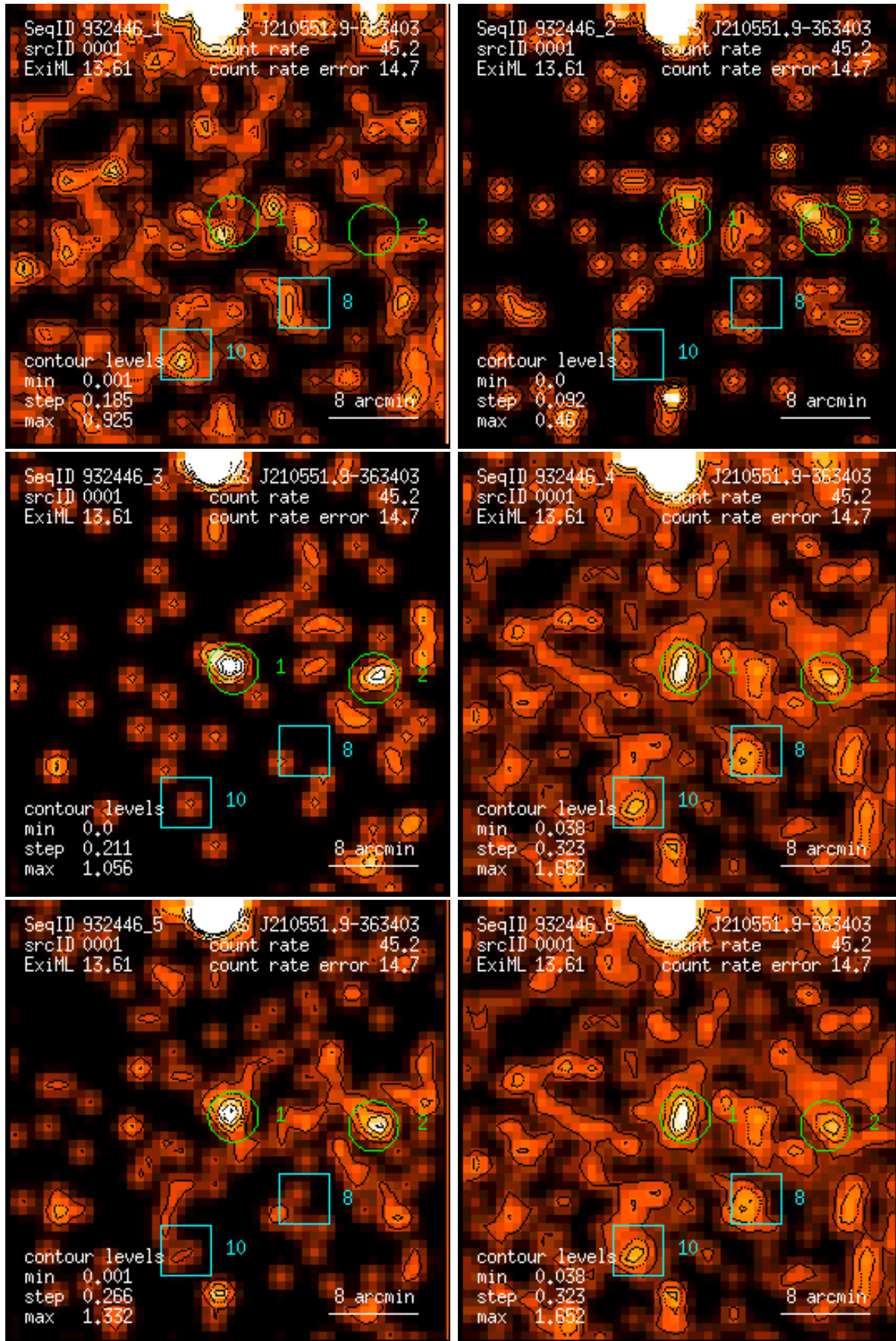
Figure 1: RASS 932446: detection 0001: band rate images, Gaussian filter: (1) PSPC channels 11 – 41, (2) 52 – 90, (3) 91 – 201, (4) 11 – 235, (5) 52 – 201, (6) 11 – 201. Broad band rates in counts/ks. Band rate contour levels in counts/ks/arcmin 2 .
