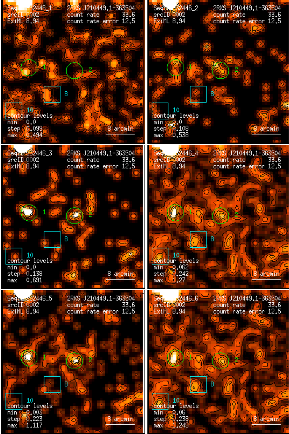
Figure 2: RASS 932446: detection 0002: band rate images, Gaussian filter: (1) PSPC channels 11 – 41, (2) 52 – 90, (3) 91 – 201, (4) 11 – 235, (5) 52 – 201, (6) 11 – 201. Broad band rates in counts/ks. Band rate contour levels in counts/ks/arcmin 2 .
