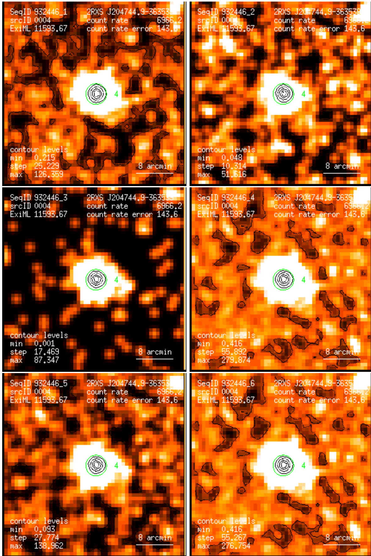
Figure 4: RASS 932446: detection 0004: band rate images, Gaussian filter: (1) PSPC channels 11 – 41, (2) 52 – 90, (3) 91 – 201, (4) 11 – 235, (5) 52 – 201, (6) 11 – 201. Broad band rates in counts/ks. Band rate contour levels in counts/ks/arcmin 2 .
