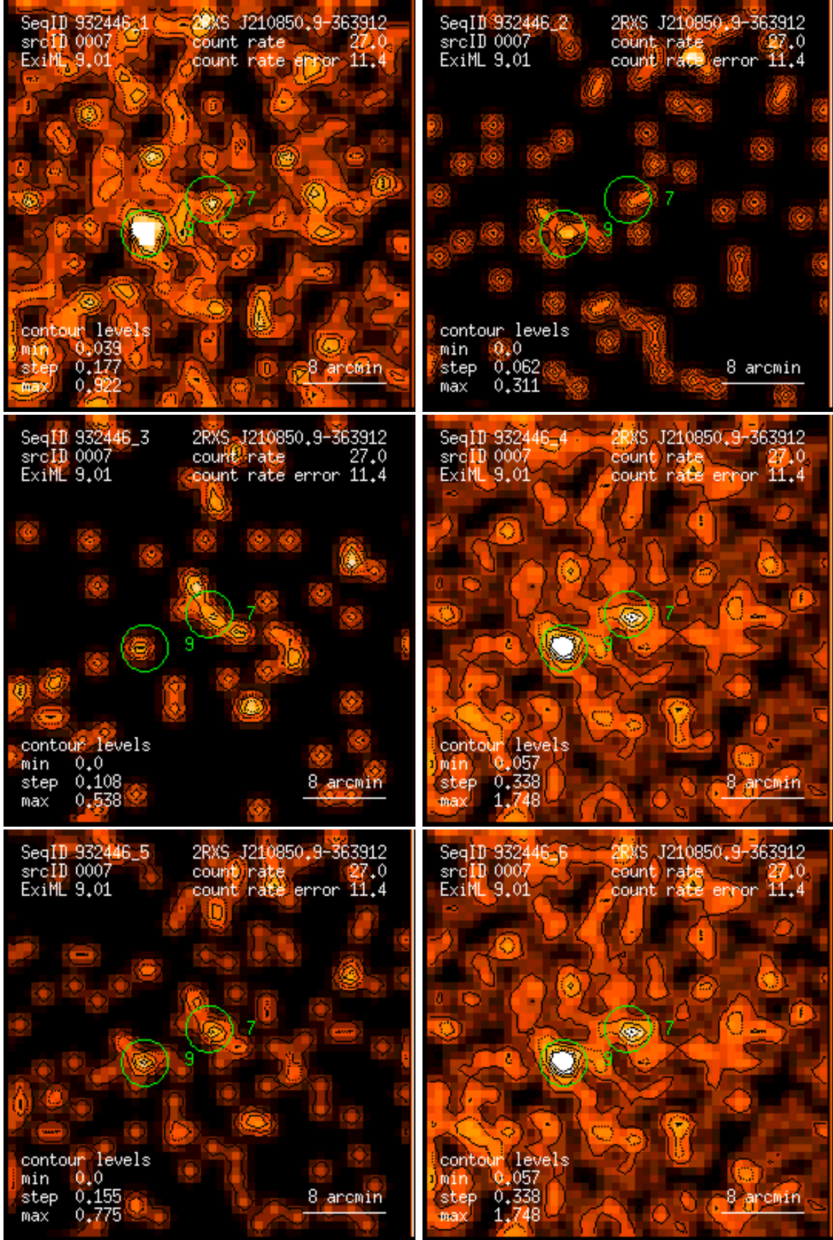
Figure 7: RASS 932446: detection 0007: band rate images, Gaussian filter: (1) PSPC channels 11 – 41, (2) 52 – 90, (3) 91 – 201, (4) 11 – 235, (5) 52 – 201, (6) 11 – 201. Broad band rates in counts/ks. Band rate contour levels in counts/ks/arcmin 2 .
