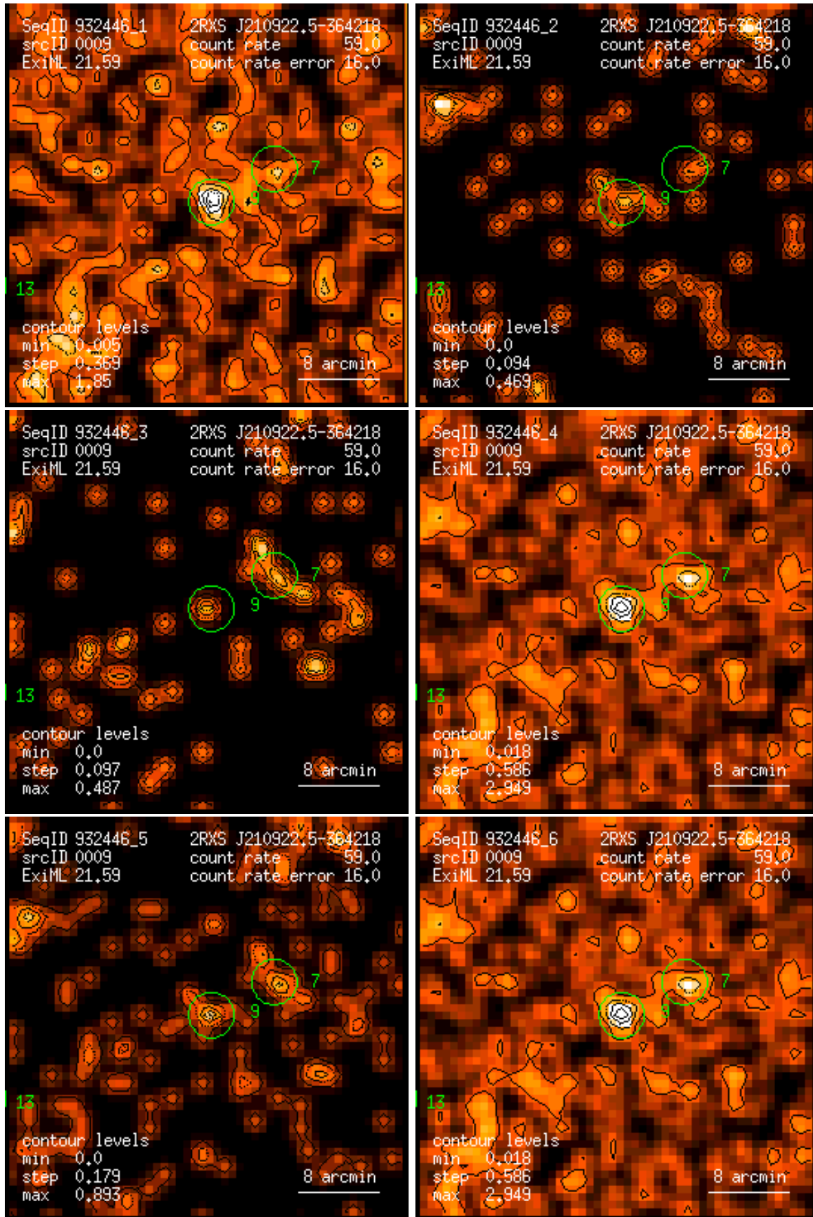
Figure 9: RASS 932446: detection 0009: band rate images, Gaussian filter: (1) PSPC channels 11 – 41, (2) 52 – 90, (3) 91 – 201, (4) 11 – 235, (5) 52 – 201, (6) 11 – 201. Broad band rates in counts/ks. Band rate contour levels in counts/ks/arcmin 2 .
