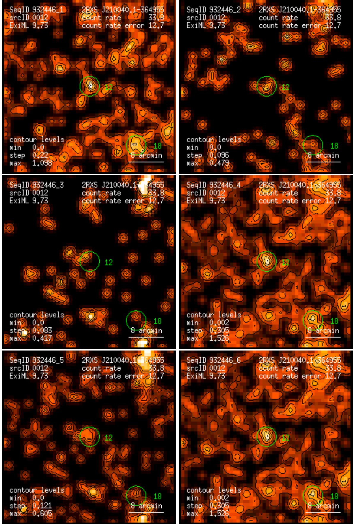
Figure 12: RASS 932446: detection 0012: band rate images, Gaussian filter: (1) PSPC channels 11 – 41, (2) 52 – 90, (3) 91 – 201, (4) 11 – 235, (5) 52 – 201, (6) 11 – 201. Broad band rates in counts/ks. Band rate contour levels in counts/ks/arcmin 2 .
