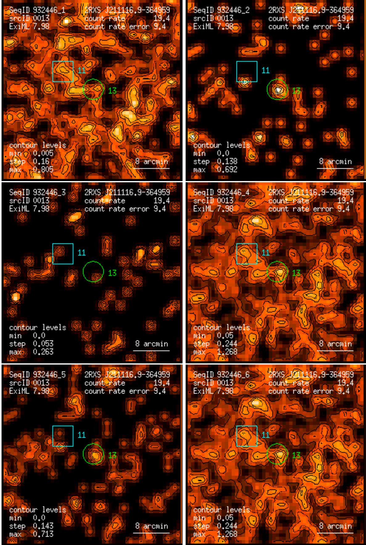
Figure 13: RASS 932446: detection 0013: band rate images, Gaussian filter: (1) PSPC channels 11 – 41, (2) 52 – 90, (3) 91 – 201, (4) 11 – 235, (5) 52 – 201, (6) 11 – 201. Broad band rates in counts/ks. Band rate contour levels in counts/ks/arcmin 2 .
