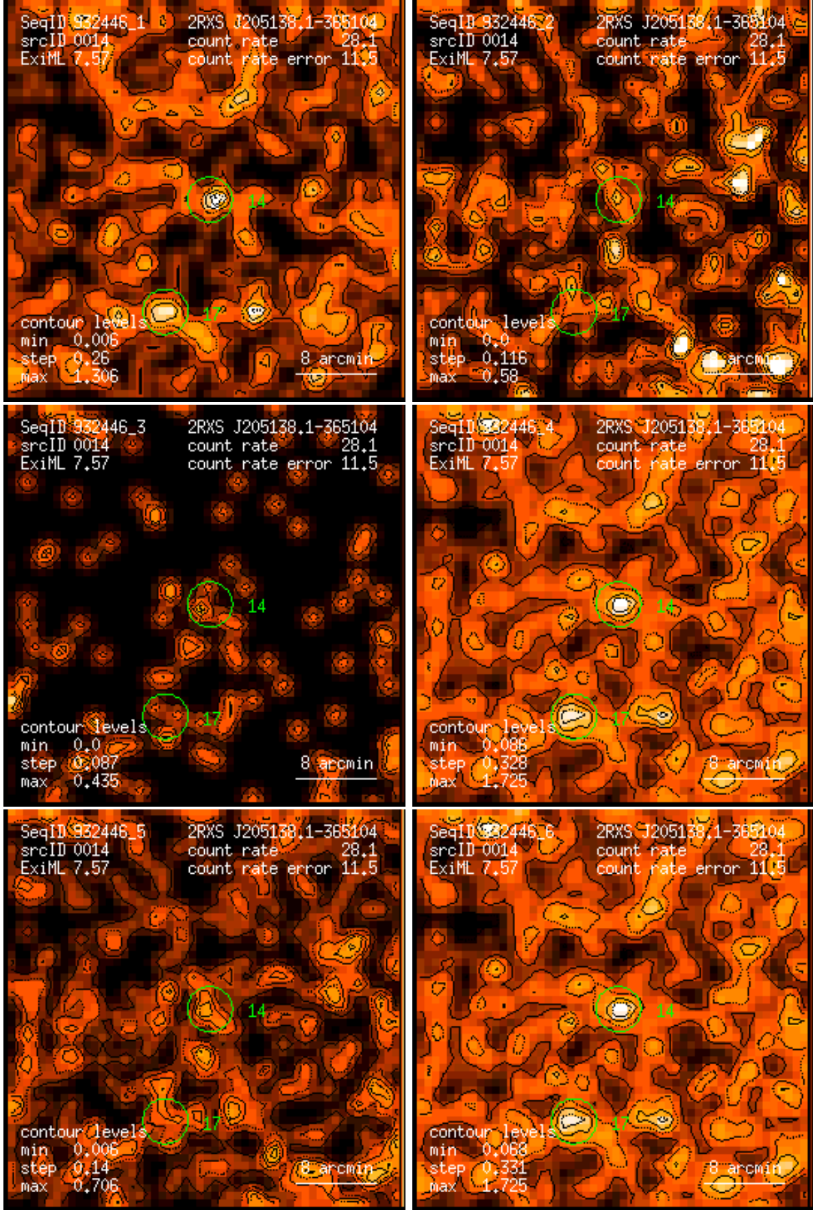
Figure 14: RASS 932446: detection 0014: band rate images, Gaussian filter: (1) PSPC channels 11 – 41, (2) 52 – 90, (3) 91 – 201, (4) 11 – 235, (5) 52 – 201, (6) 11 – 201. Broad band rates in counts/ks. Band rate contour levels in counts/ks/arcmin 2 .
