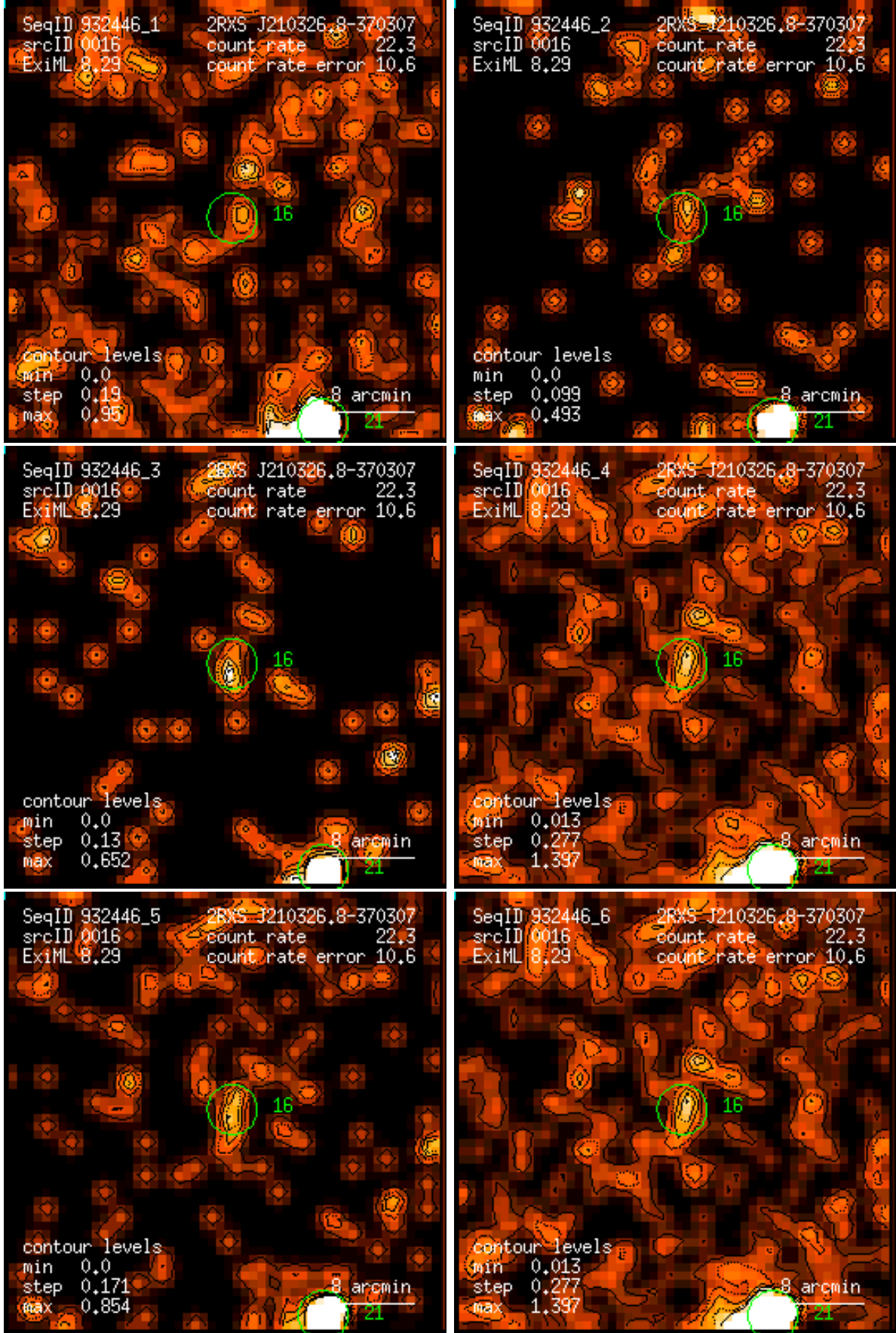
Figure 16: RASS 932446: detection 0016: band rate images, Gaussian filter: (1) PSPC channels 11 – 41, (2) 52 – 90, (3) 91 – 201, (4) 11 – 235, (5) 52 – 201, (6) 11 – 201. Broad band rates in counts/ks. Band rate contour levels in counts/ks/arcmin 2 .
