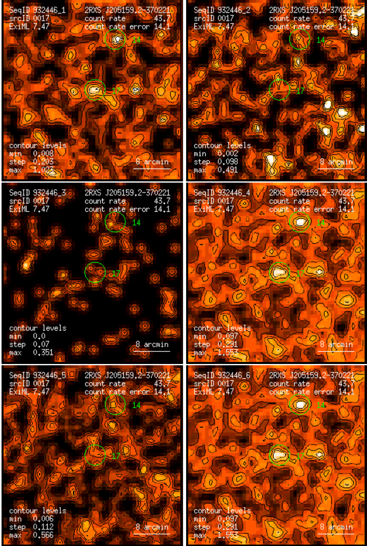
Figure 17: RASS 932446: detection 0017: band rate images, Gaussian filter: (1) PSPC channels 11 – 41, (2) 52 – 90, (3) 91 – 201, (4) 11 – 235, (5) 52 – 201, (6) 11 – 201. Broad band rates in counts/ks. Band rate contour levels in counts/ks/arcmin 2 .
