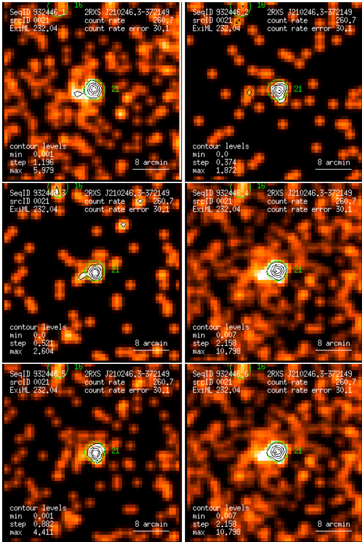
Figure 21: RASS 932446: detection 0021: band rate images, Gaussian filter: (1) PSPC channels 11 – 41, (2) 52 – 90, (3) 91 – 201, (4) 11 – 235, (5) 52 – 201, (6) 11 – 201. Broad band rates in counts/ks. Band rate contour levels in counts/ks/arcmin 2 .
