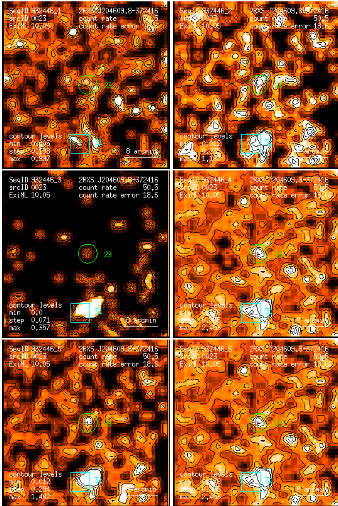
Figure 23: RASS 932446: detection 0023: band rate images, Gaussian filter: (1) PSPC channels 11 – 41, (2) 52 – 90, (3) 91 – 201, (4) 11 – 235, (5) 52 – 201, (6) 11 – 201. Broad band rates in counts/ks. Band rate contour levels in counts/ks/arcmin 2 .
