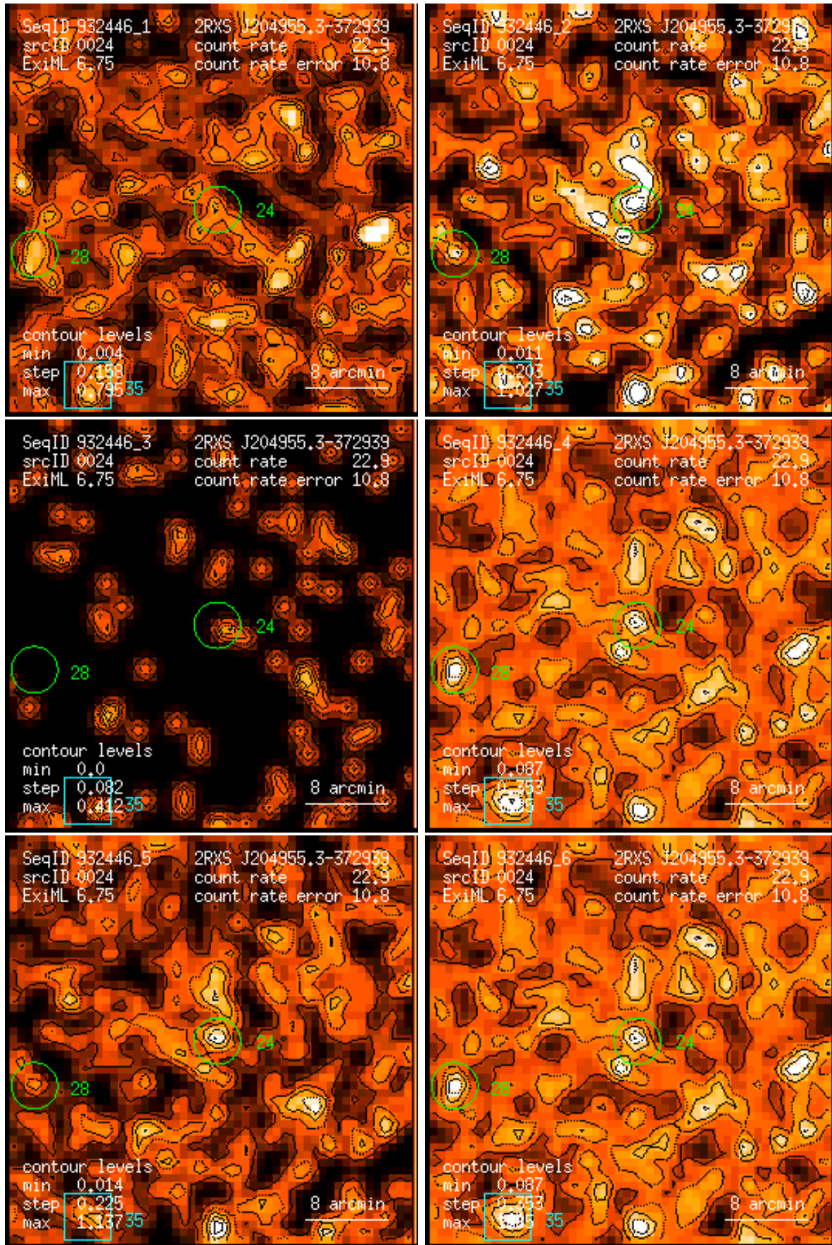
Figure 24: RASS 932446: detection 0024: band rate images, Gaussian filter: (1) PSPC channels 11 – 41, (2) 52 – 90, (3) 91 – 201, (4) 11 – 235, (5) 52 – 201, (6) 11 – 201. Broad band rates in counts/ks. Band rate contour levels in counts/ks/arcmin 2 .
