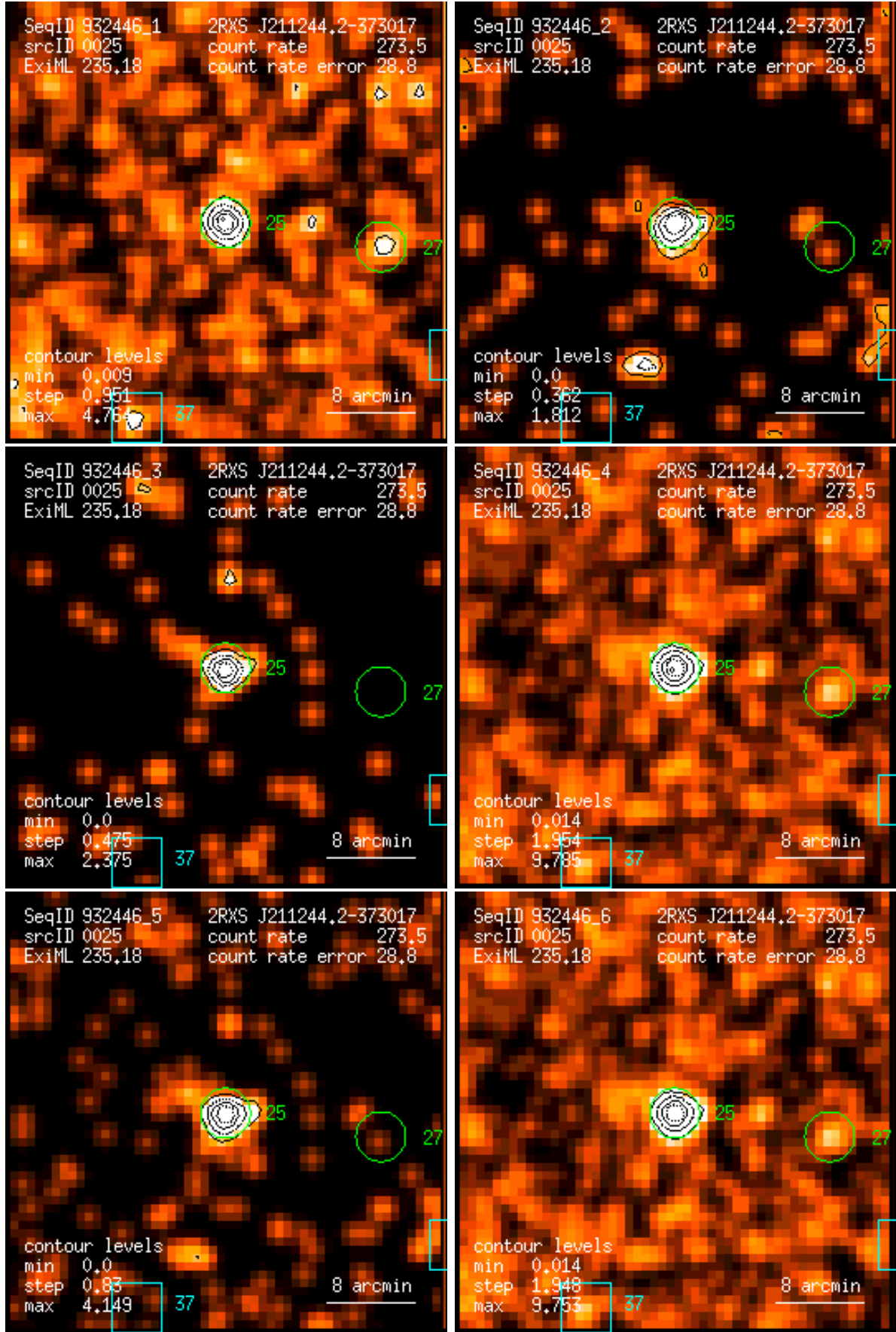
Figure 25: RASS 932446: detection 0025: band rate images, Gaussian filter: (1) PSPC channels 11 – 41, (2) 52 – 90, (3) 91 – 201, (4) 11 – 235, (5) 52 – 201, (6) 11 – 201. Broad band rates in counts/ks. Band rate contour levels in counts/ks/arcmin 2 .
