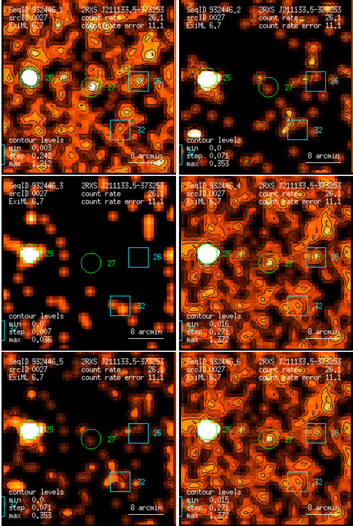
Figure 27: RASS 932446: detection 0027: band rate images, Gaussian filter: (1) PSPC channels 11 – 41, (2) 52 – 90, (3) 91 – 201, (4) 11 – 235, (5) 52 – 201, (6) 11 – 201. Broad band rates in counts/ks. Band rate contour levels in counts/ks/arcmin 2 .
