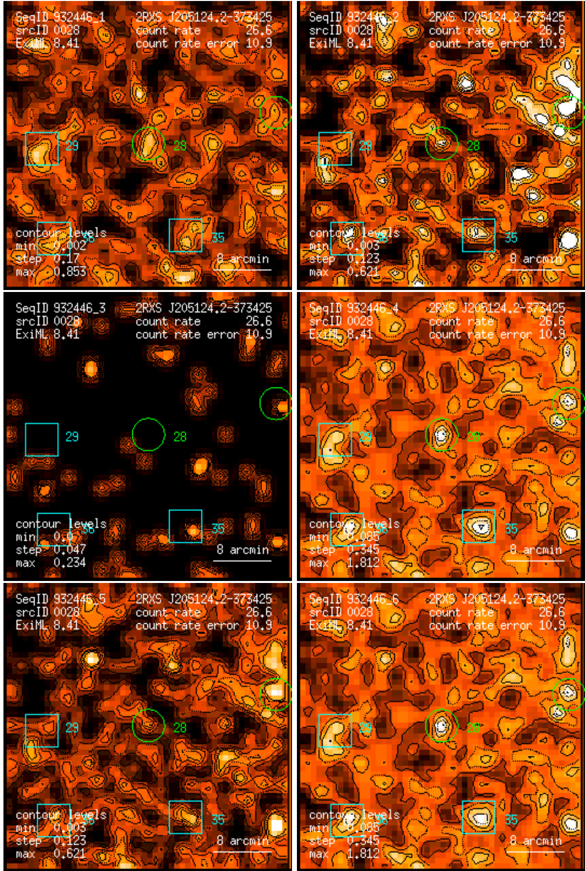
Figure 28: RASS 932446: detection 0028: band rate images, Gaussian filter: (1) PSPC channels 11 – 41, (2) 52 – 90, (3) 91 – 201, (4) 11 – 235, (5) 52 – 201, (6) 11 – 201. Broad band rates in counts/ks. Band rate contour levels in counts/ks/arcmin 2 .
