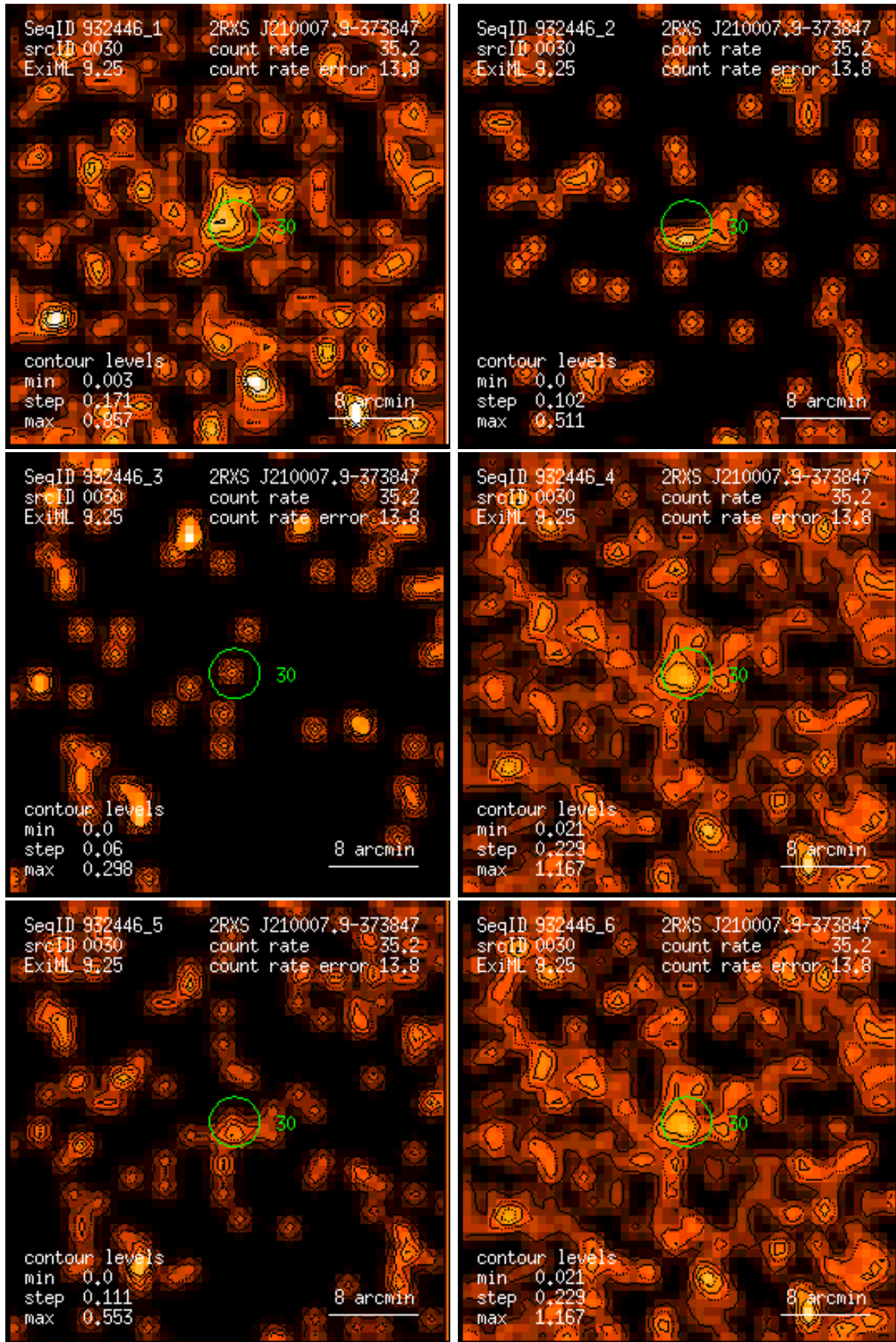
Figure 30: RASS 932446: detection 0030: band rate images, Gaussian filter: (1) PSPC channels 11 – 41, (2) 52 – 90, (3) 91 – 201, (4) 11 – 235, (5) 52 – 201, (6) 11 – 201. Broad band rates in counts/ks. Band rate contour levels in counts/ks/arcmin 2 .
