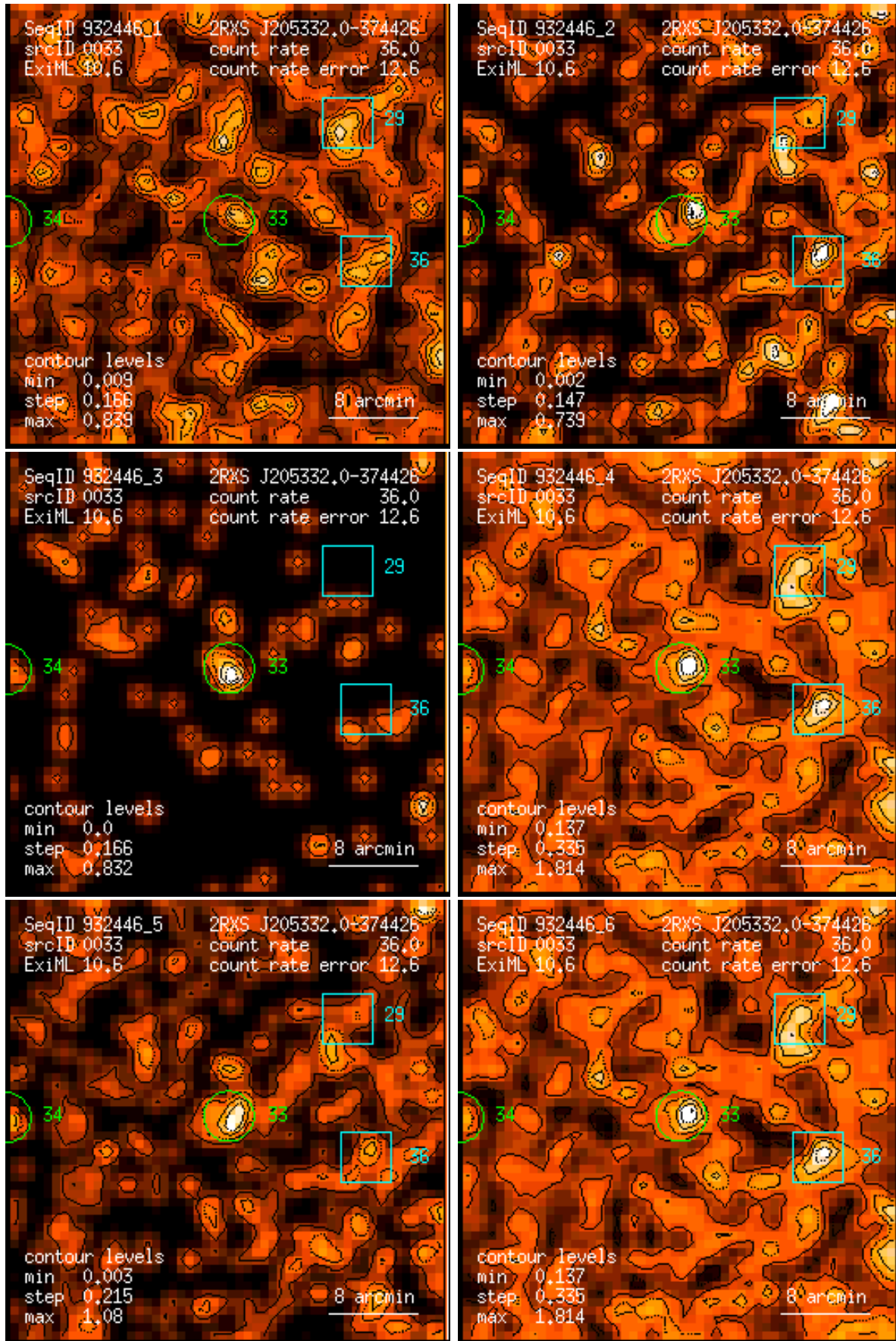
Figure 33: RASS 932446: detection 0033: band rate images, Gaussian filter: (1) PSPC channels 11 – 41, (2) 52 – 90, (3) 91 – 201, (4) 11 – 235, (5) 52 – 201, (6) 11 – 201. Broad band rates in counts/ks. Band rate contour levels in counts/ks/arcmin 2 .
