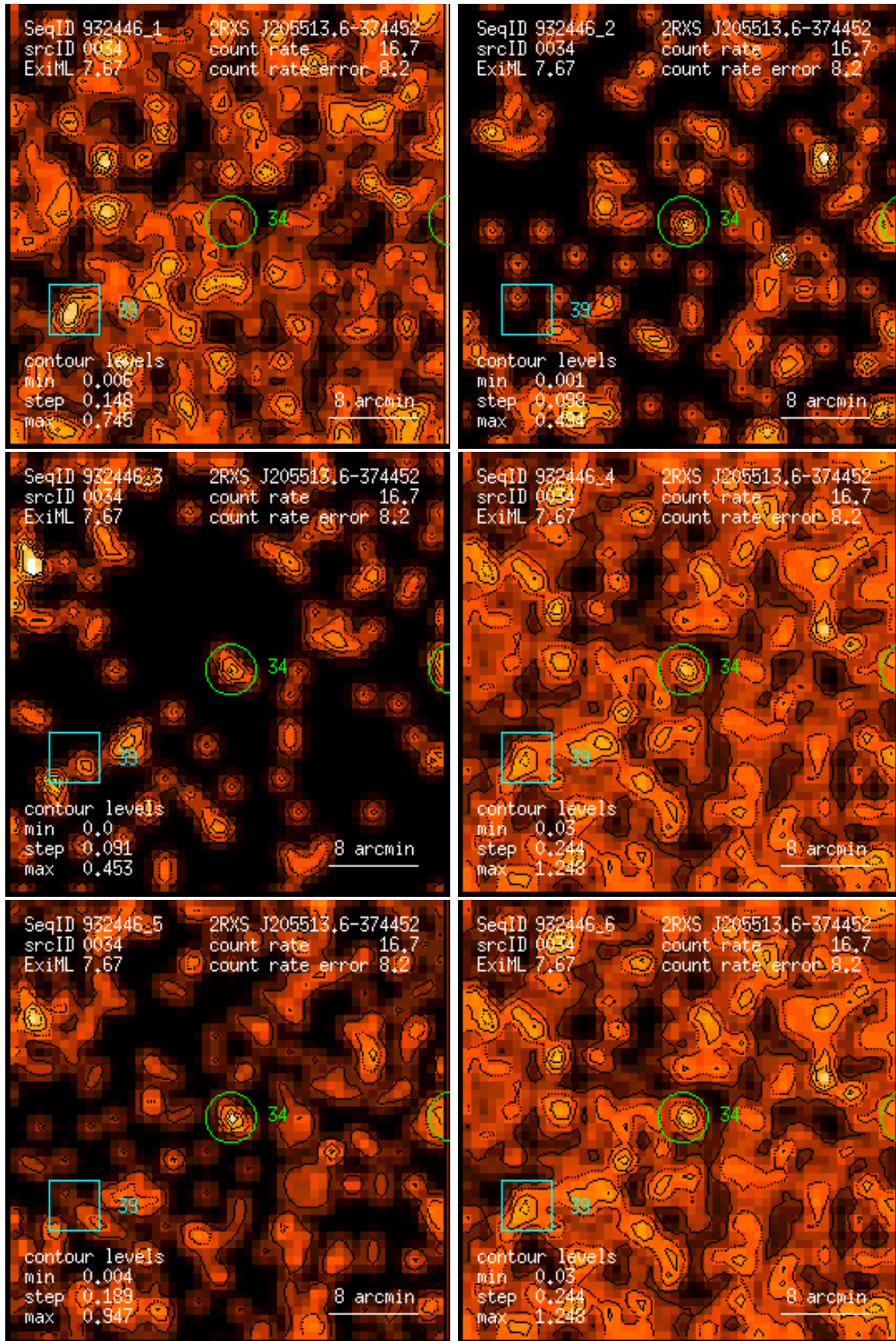
Figure 34: RASS 932446: detection 0034: band rate images, Gaussian filter: (1) PSPC channels 11 – 41, (2) 52 – 90, (3) 91 – 201, (4) 11 – 235, (5) 52 – 201, (6) 11 – 201. Broad band rates in counts/ks. Band rate contour levels in counts/ks/arcmin 2 .
