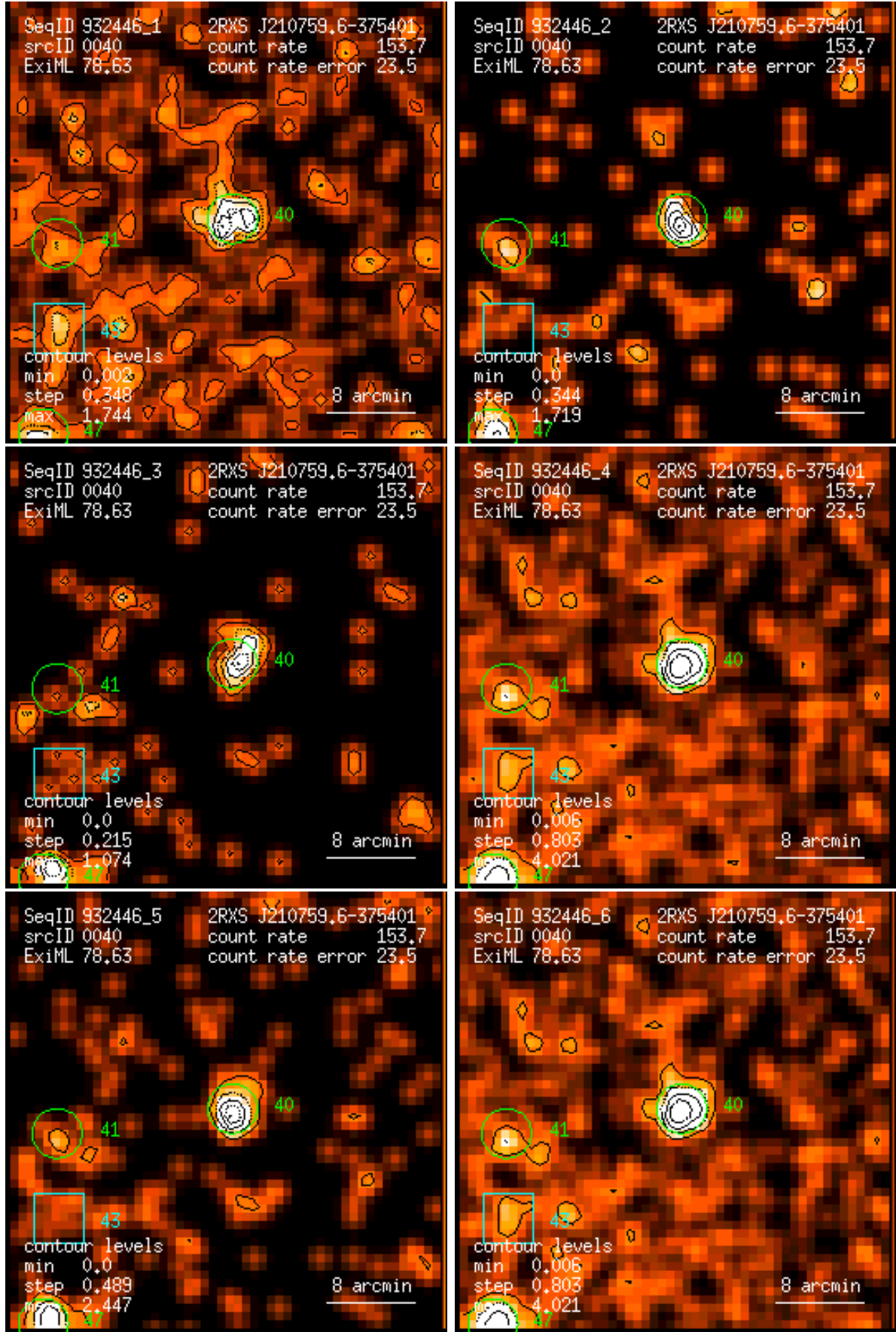
Figure 40: RASS 932446: detection 0040: band rate images, Gaussian filter: (1) PSPC channels 11 – 41, (2) 52 – 90, (3) 91 – 201, (4) 11 – 235, (5) 52 – 201, (6) 11 – 201. Broad band rates in counts/ks. Band rate contour levels in counts/ks/arcmin 2 .
