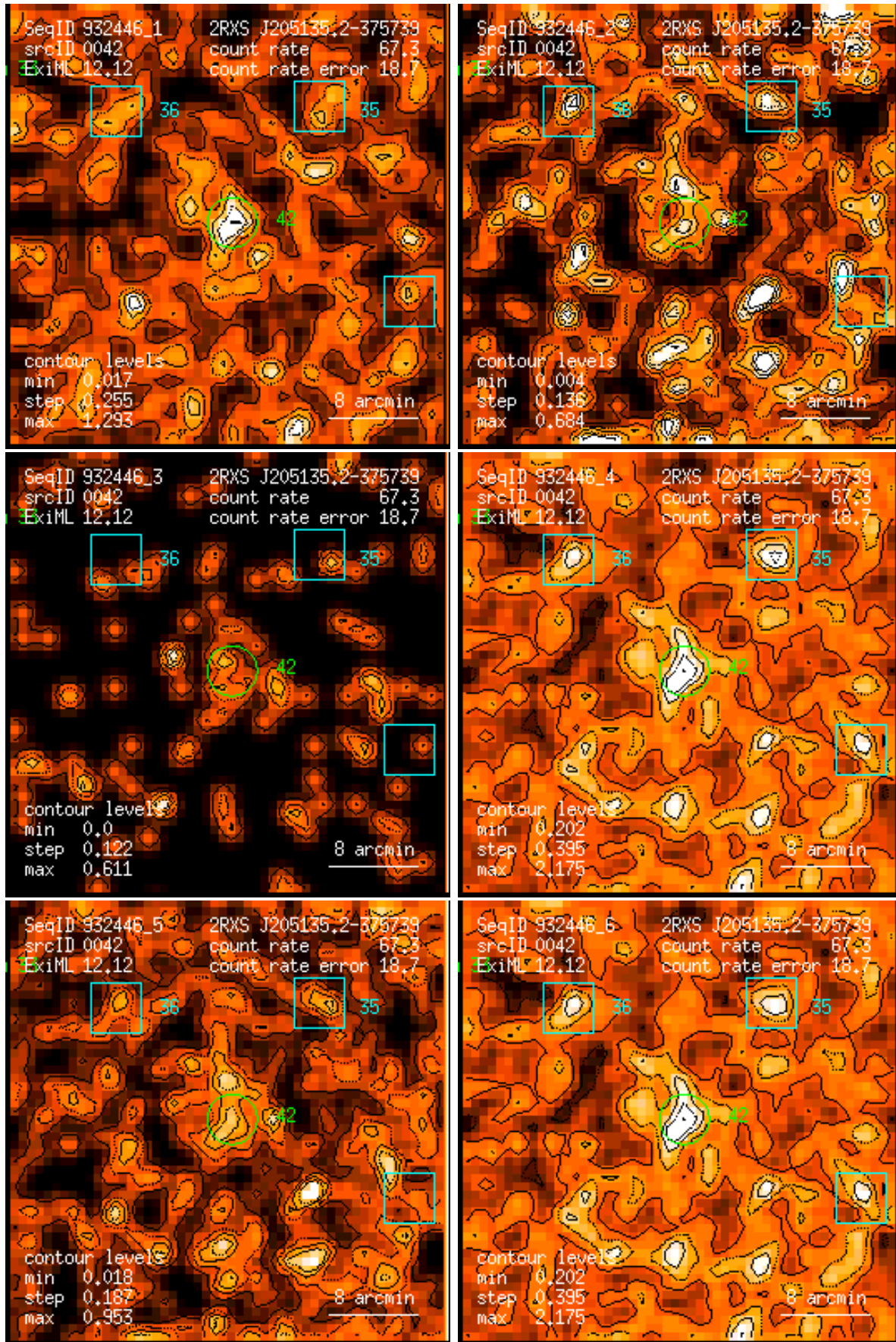
Figure 42: RASS 932446: detection 0042: band rate images, Gaussian filter: (1) PSPC channels 11 – 41, (2) 52 – 90, (3) 91 – 201, (4) 11 – 235, (5) 52 – 201, (6) 11 – 201. Broad band rates in counts/ks. Band rate contour levels in counts/ks/arcmin 2 .
