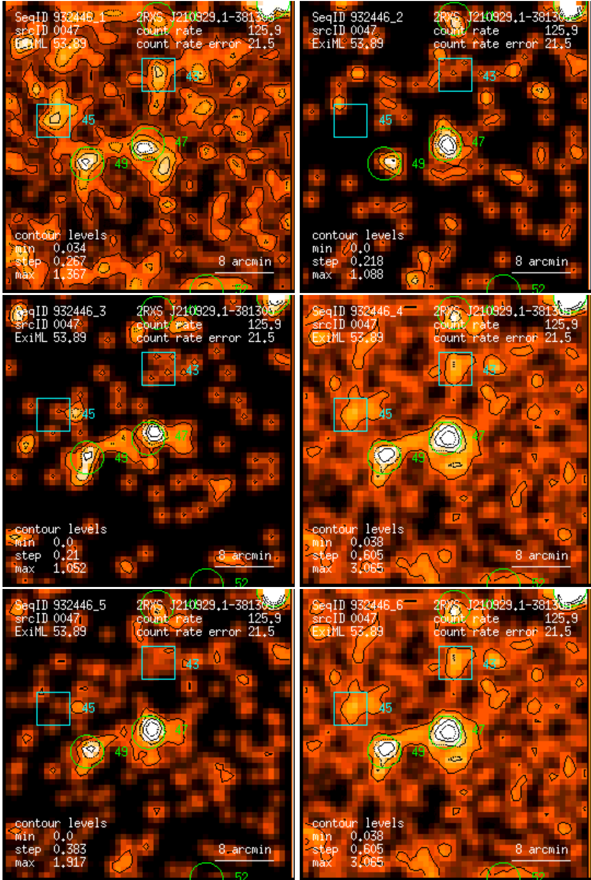
Figure 47: RASS 932446: detection 0047: band rate images, Gaussian filter: (1) PSPC channels 11 – 41, (2) 52 – 90, (3) 91 – 201, (4) 11 – 235, (5) 52 – 201, (6) 11 – 201. Broad band rates in counts/ks. Band rate contour levels in counts/ks/arcmin 2 .
